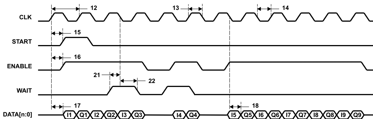
Figure 5-85. uPP Double Data Rate (DDR) Transmit Timing
