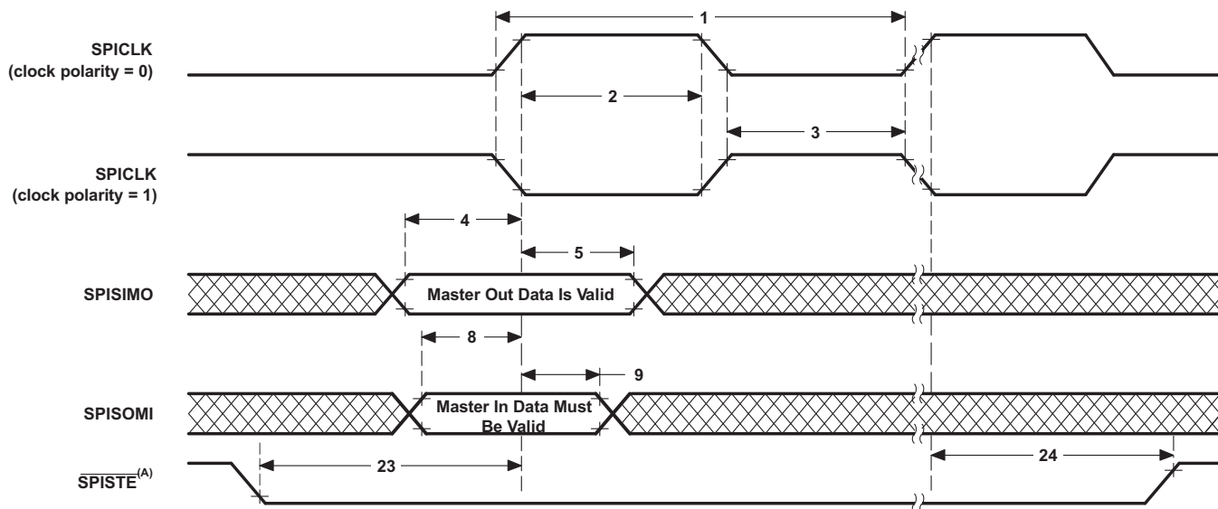
图 5-75. High-Speed SPI Master Mode External Timing (Clock Phase = 0)
