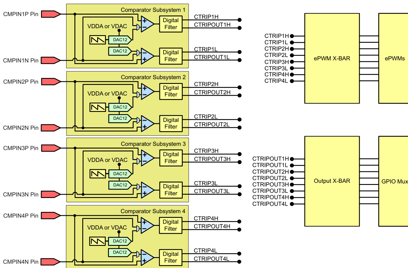
图 5-38. CMPSS Connectivity (100-Pin PZP)
