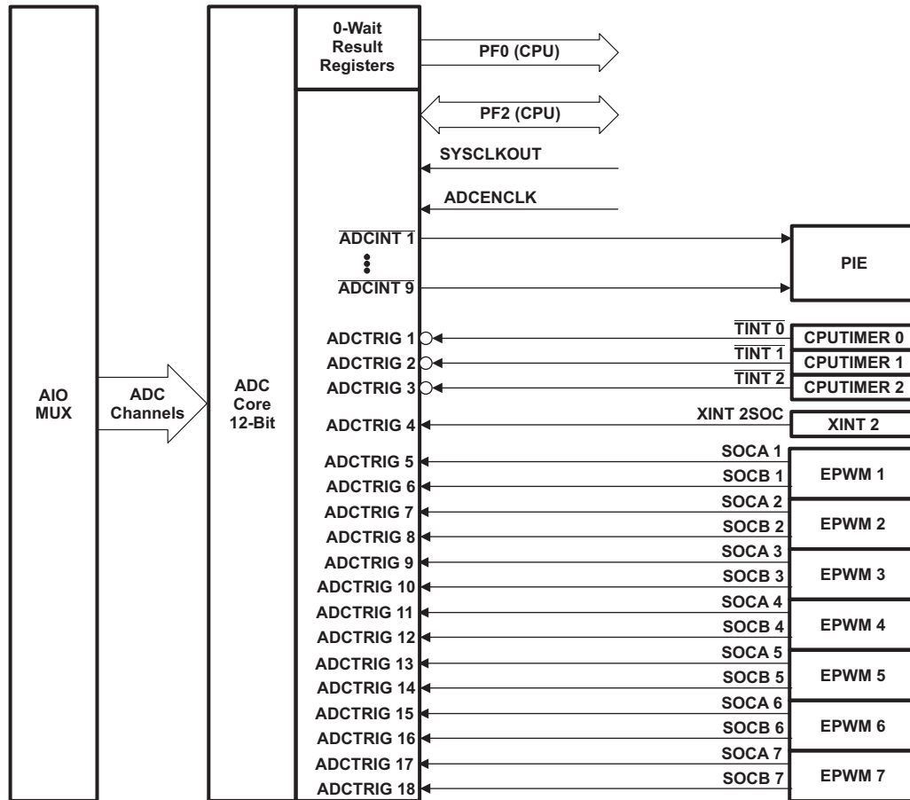
Figure 6-17. ADC Connections
