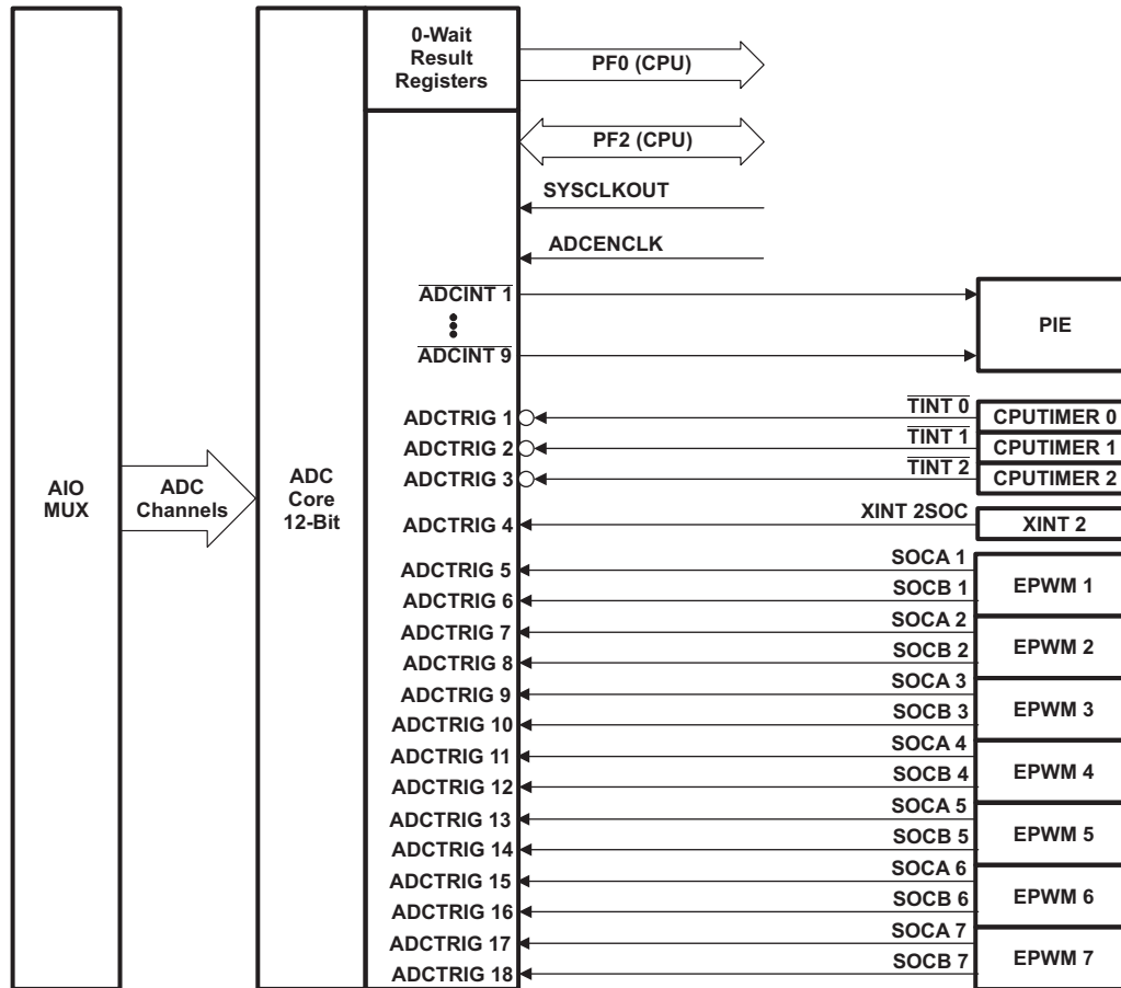
Figure 5-14. ADC Connections
