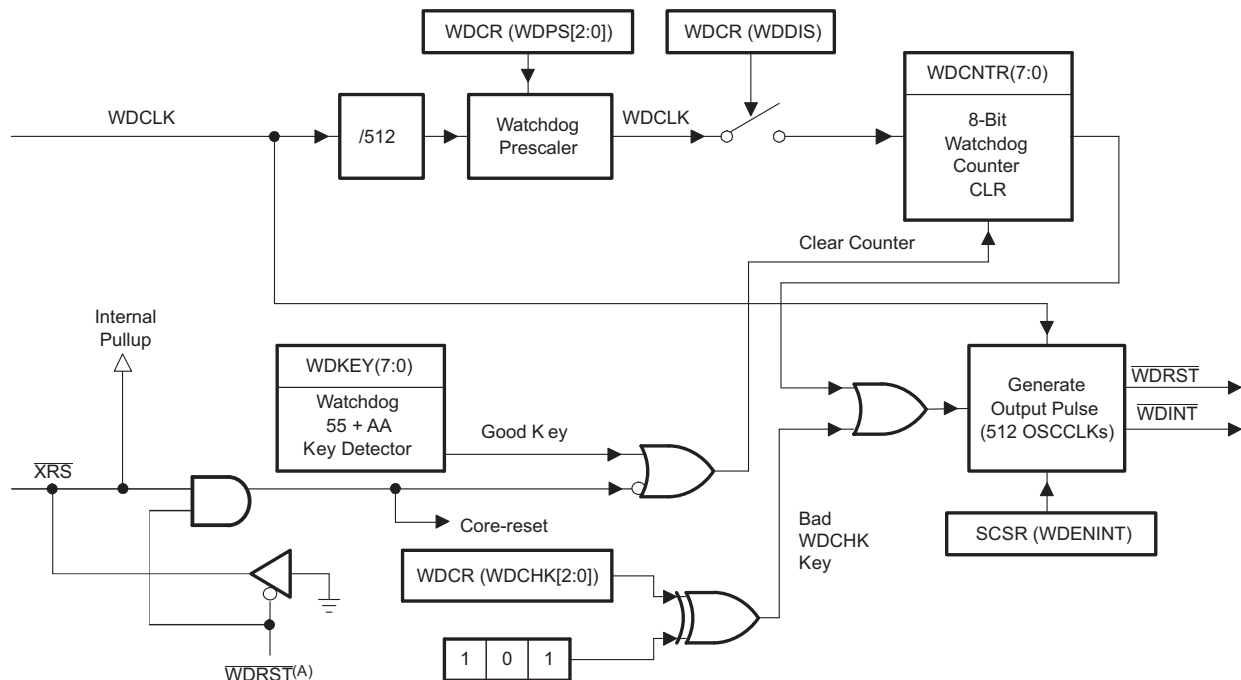
Figure 5-8. CPU-watchdog Module
