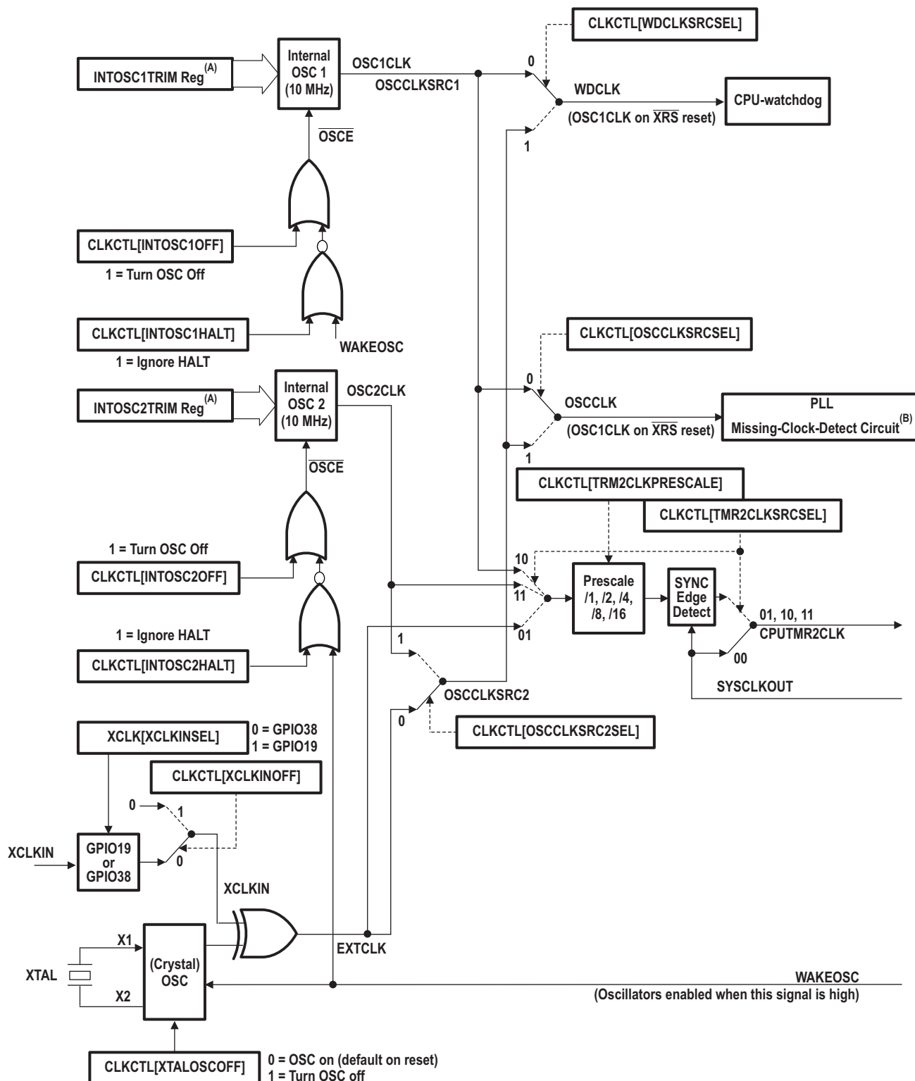
Figure 5-4. Clock Tree
