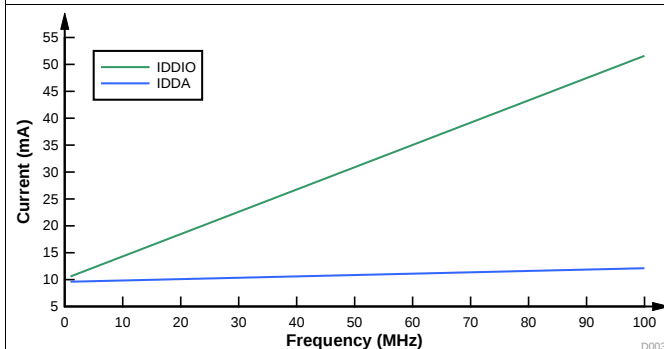
图 5-4. Current Versus Frequency — DCDC
