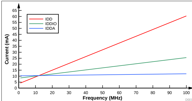
图 5-2. Current Versus Frequency — External Supply
