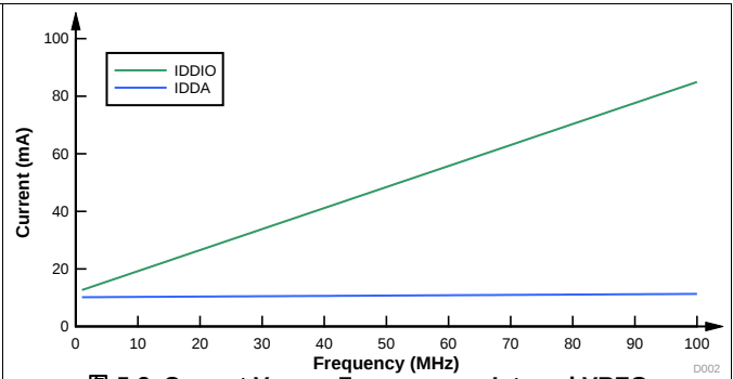
图 5-3. Current Versus Frequency — Internal VREG
