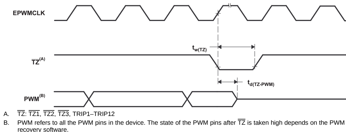
图 5-61. PWM Hi-Z Characteristics
