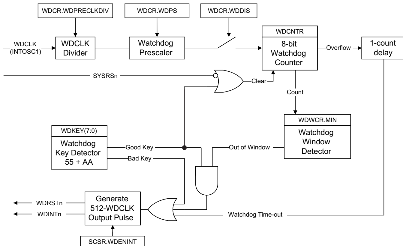
图 6-4. Windowed Watchdog
