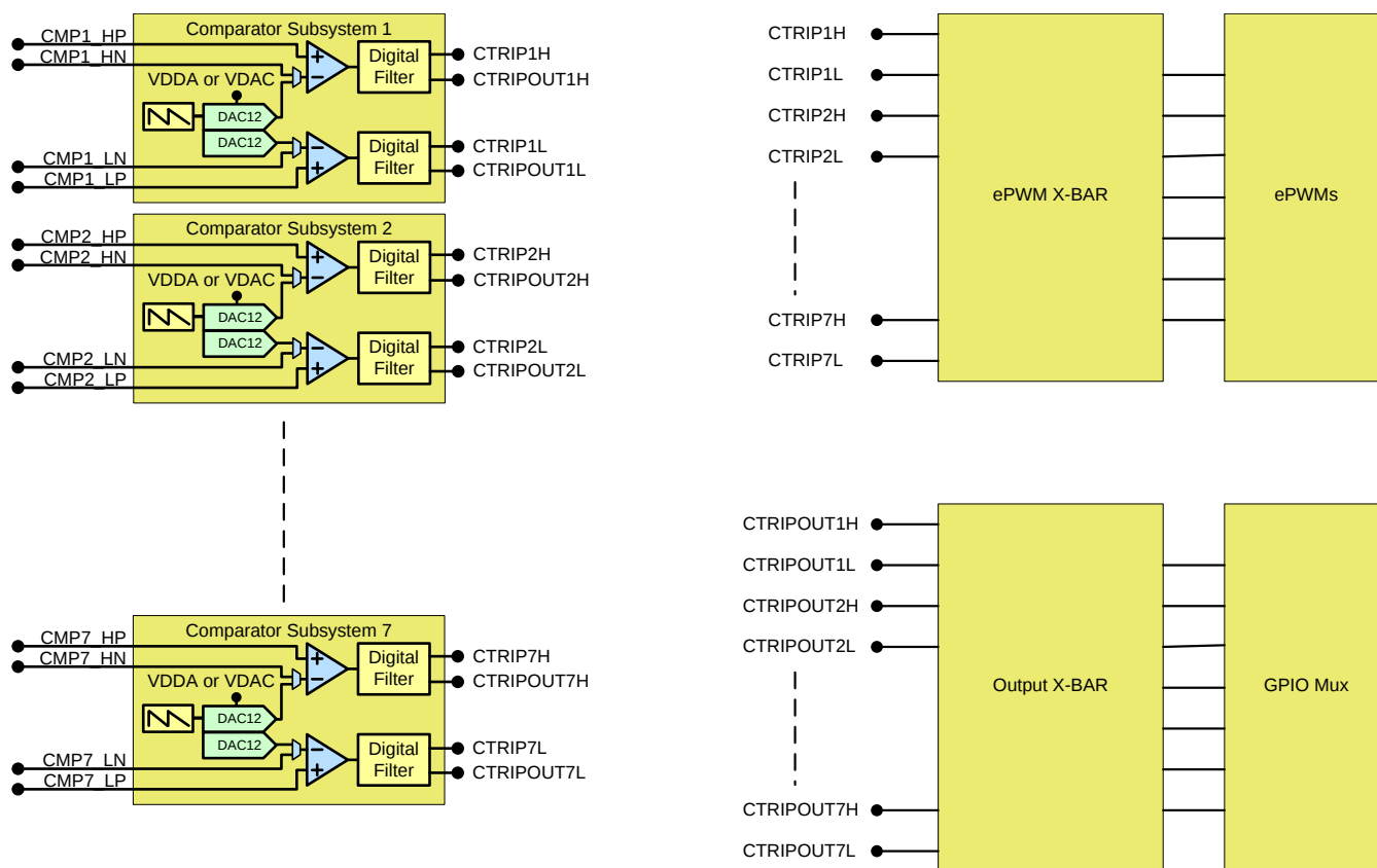
图 5-48. CMPSS Connectivity
