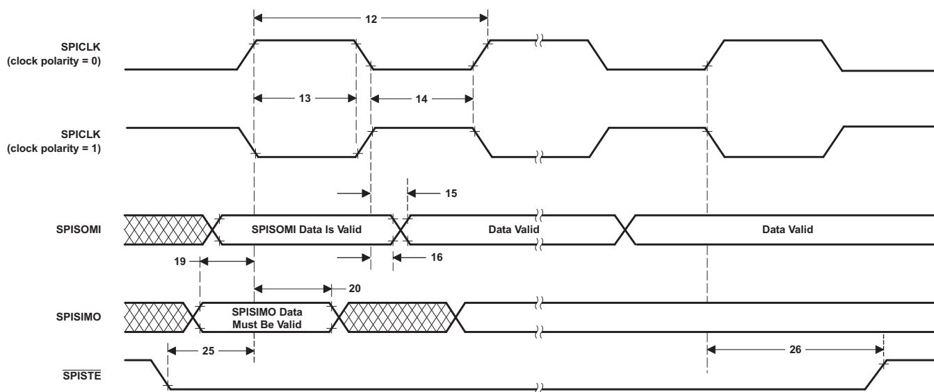
图 5-74. High-Speed SPI Slave Mode External Timing (Clock Phase = 1)
