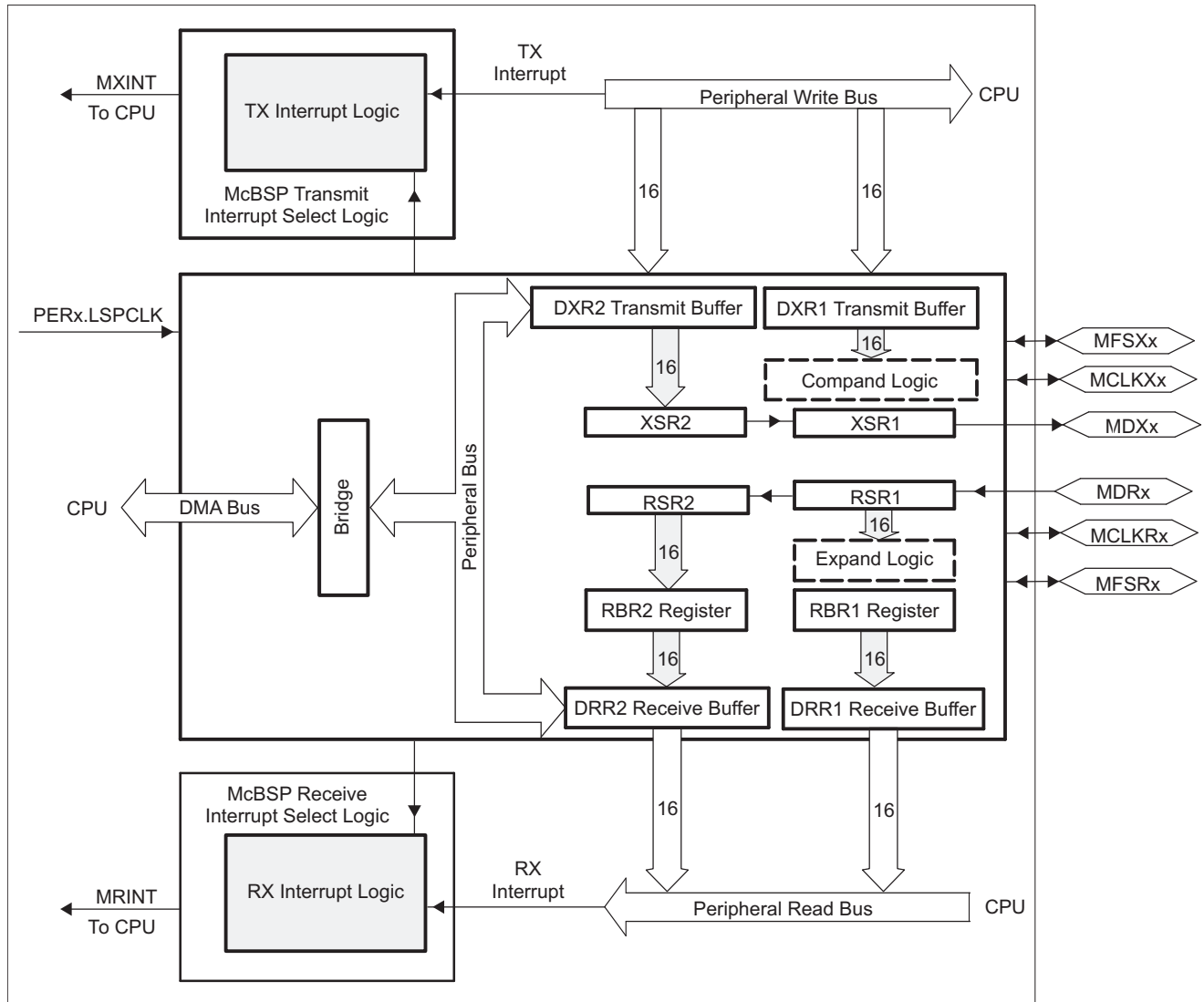
图 5-58. McBSP Block Diagram
