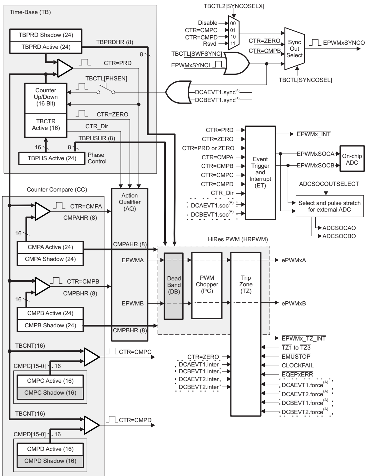
图 5-45. ePWM Submodules and Critical Internal Signal Interconnects
