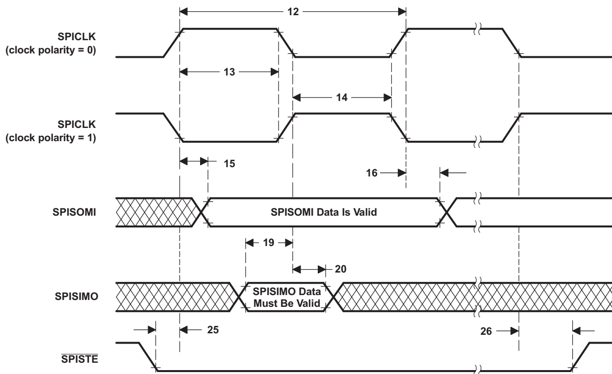
图 5-69. SPI Slave Mode External Timing (Clock Phase = 0)
