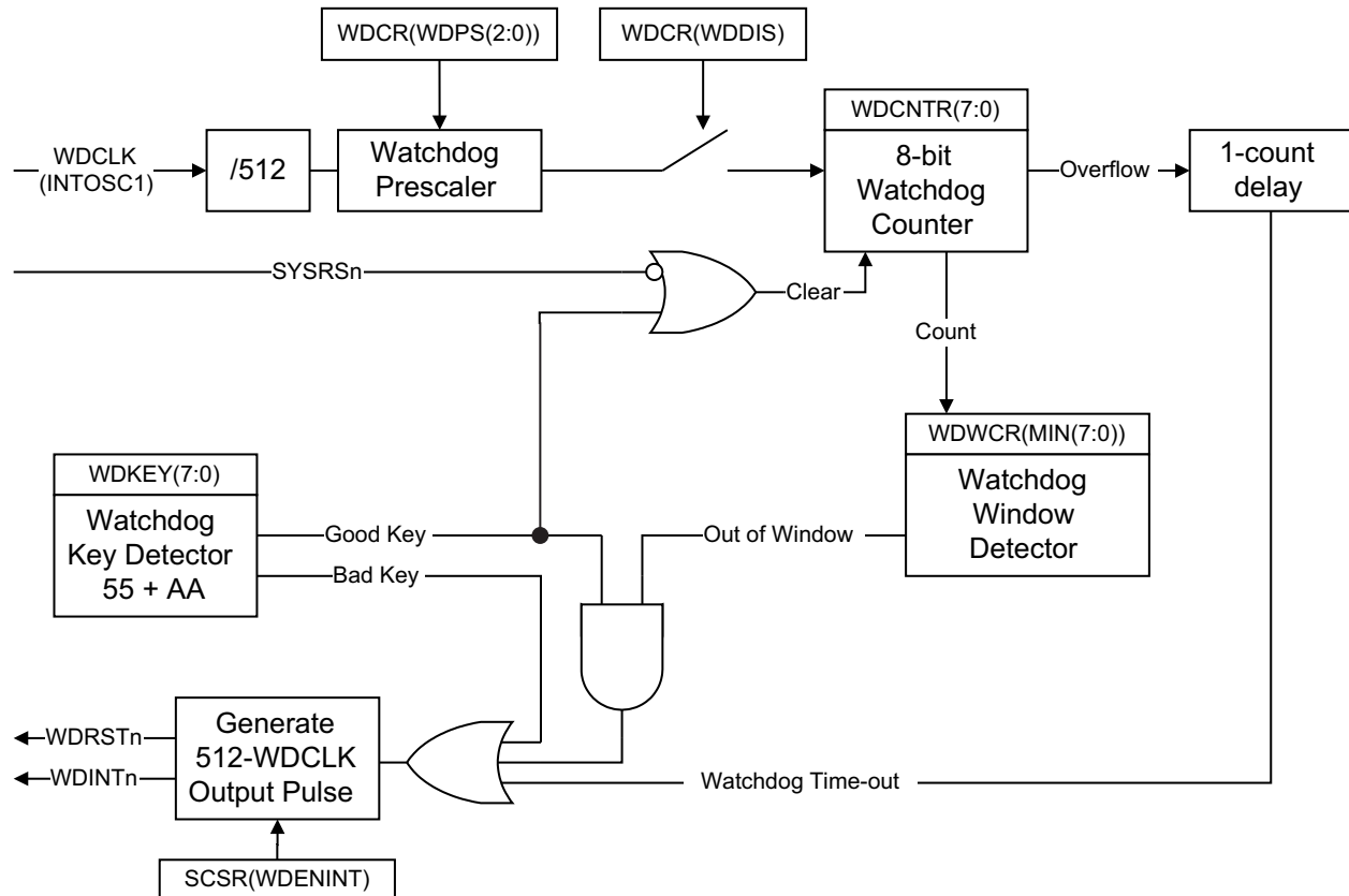
图 6-4. Windowed Watchdog
