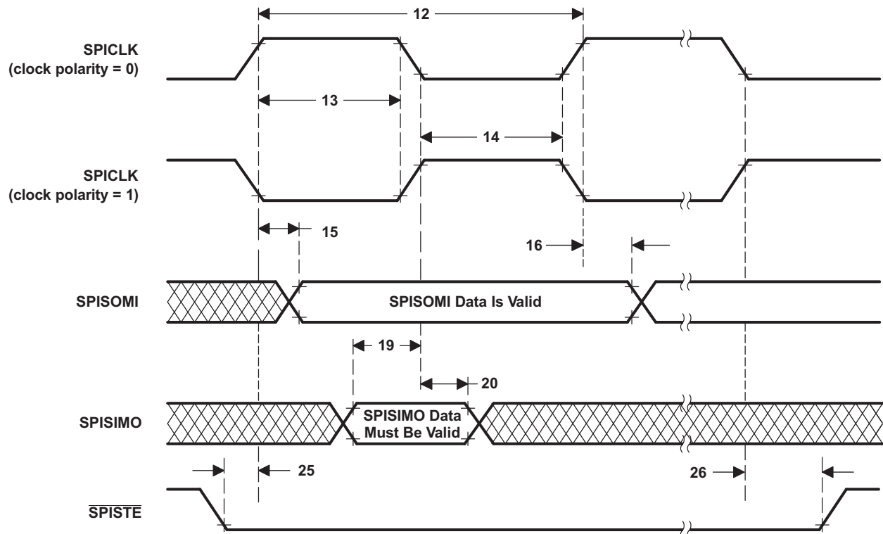
图 5-73. High-Speed SPI Slave Mode External Timing (Clock Phase = 0)
