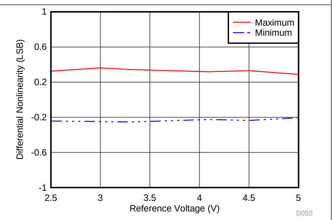
图 10. DNL vs Reference Voltage
