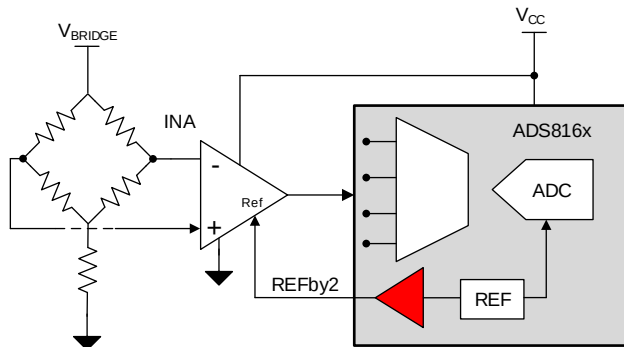
Configuration 4: High Impedance Sensor Interface with INA
