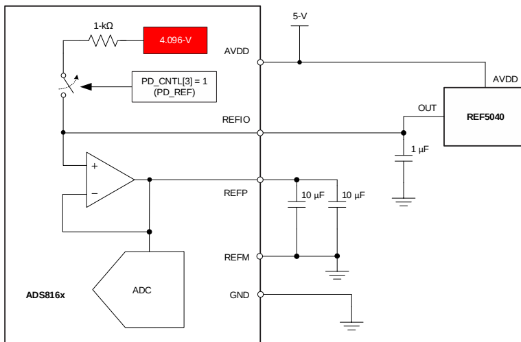
图 36. Device Connections for Using an External Reference
