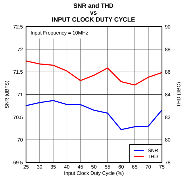
Figure 6-14. Performance Across Input Clock Duty Cycle
