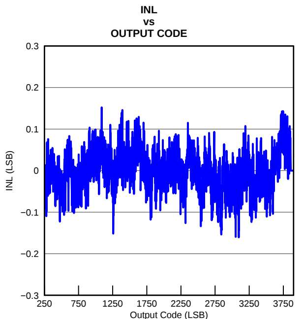
Figure 6-17. INL Plot
