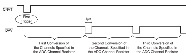
Figure 85. ADC External Trigger
