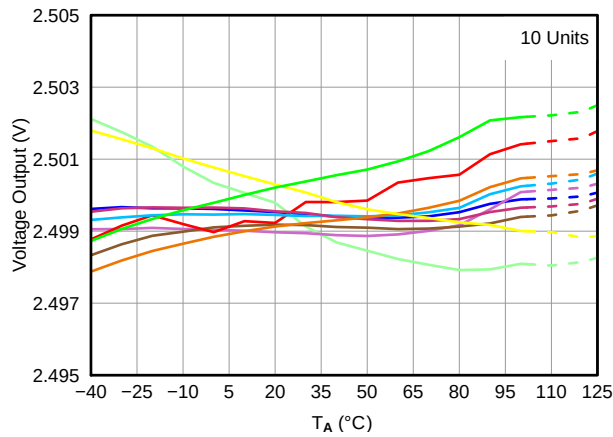
Figure 69. OUTPUT VOLTAGE vs TEMPERATURE
