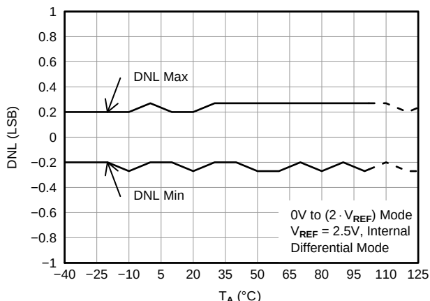
Figure 54. DIFFERENTIAL LINEARITY ERROR vs TEMPERATURE
