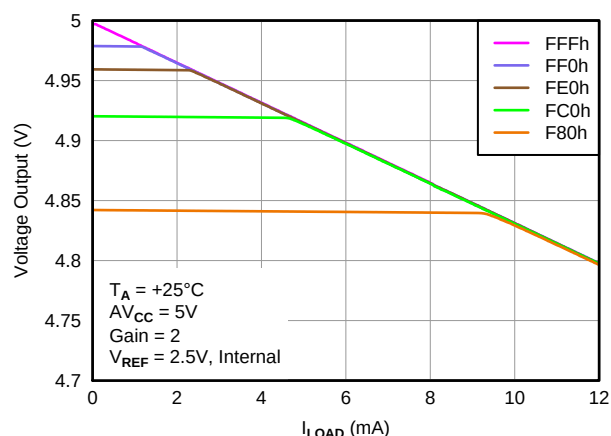
Figure 33. OUTPUT VOLTAGE vs SOURCE CURRENT CAPABILITY
