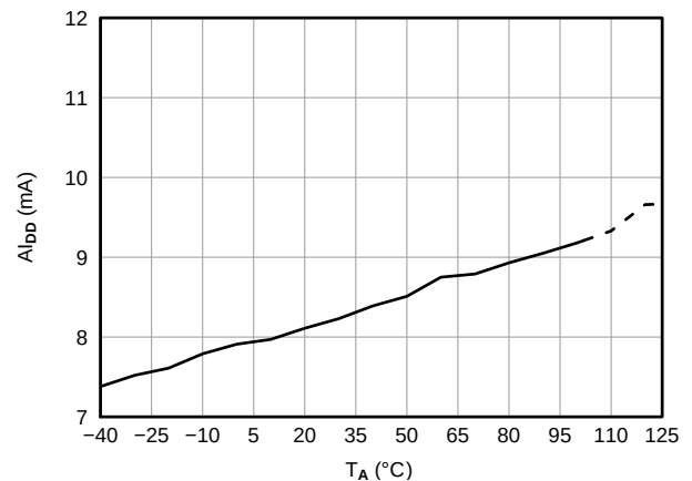
Figure 66. SUPPLY CURRENT vs TEMPERATURE
