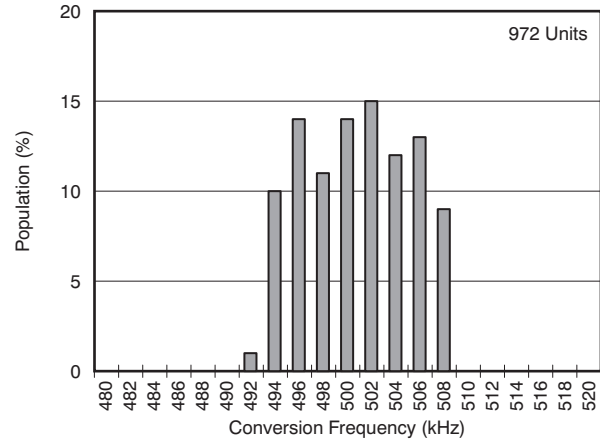
Figure 62. CONVERSION FREQUENCY
