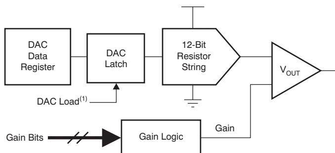
Figure 91. DAC Block Diagram
