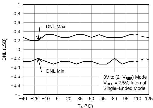
Figure 52. DIFFERENTIAL LINEARITY ERROR vs TEMPERATURE
