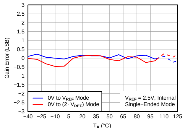
Figure 60. GAIN ERROR vs TEMPERATURE
