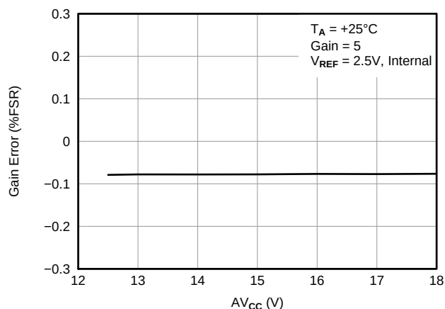
Figure 25. GAIN ERROR vs SUPPLY
