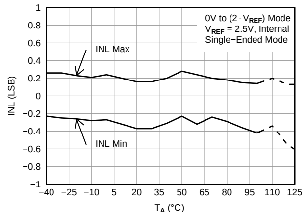
Figure 56. LINEARITY ERROR vs TEMPERATURE
