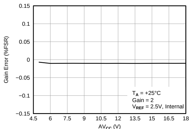
Figure 24. GAIN ERROR vs SUPPLY
