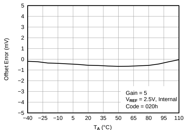
Figure 29. OFFSET VOLTAGE vs TEMPERATURE
