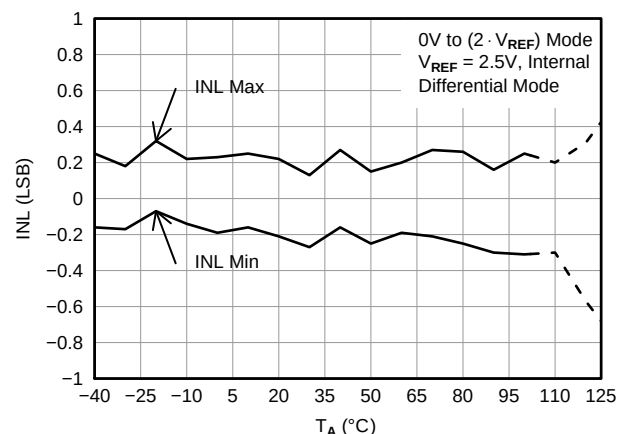
Figure 58. LINEARITY ERROR vs TEMPERATURE
