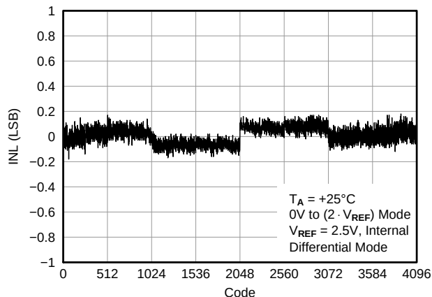
Figure 50. LINEARITY ERROR vs CODE
