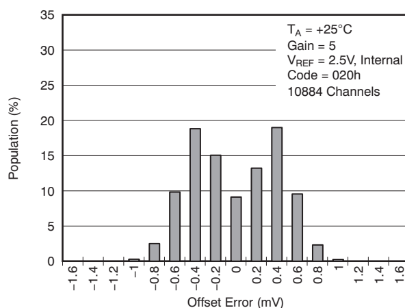
Figure 27. OFFSET VOLTAGE
