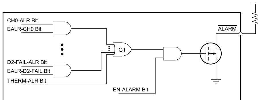
Figure 97. \overline{\text{ALARM}} Pin
