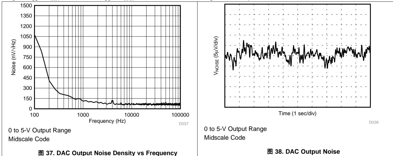
图 37. DAC Output Noise Density vs Frequency
