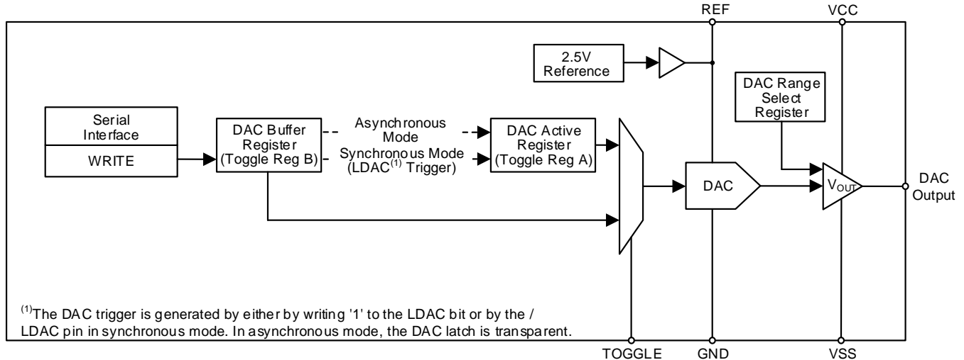
图 47. DACx1416 DAC Block Diagram
