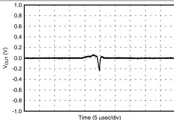
Power-down to Active DAC Mode \pm 20\text{-V} Output Range
