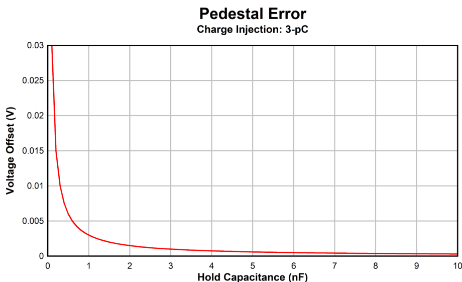
图 16. Sample and Hold Pedestal Error
