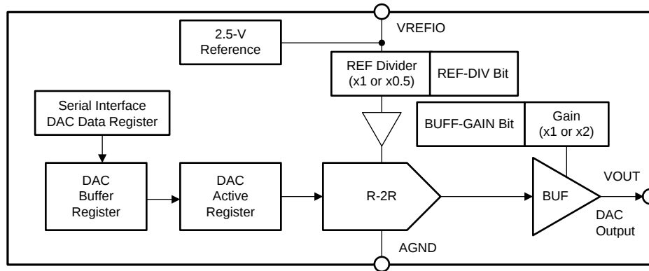
图 3. DACx0501 DAC Block Diagram
