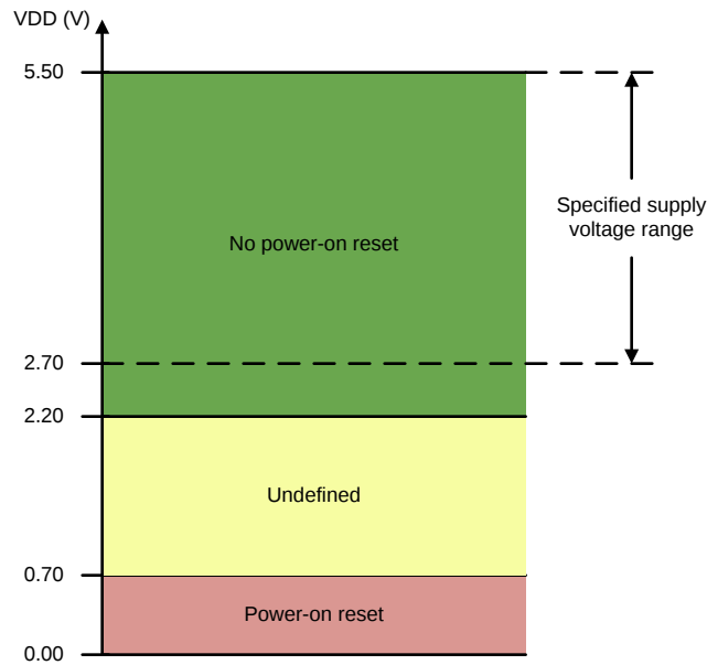
图 4. Threshold Levels for VDD POR Circuit
