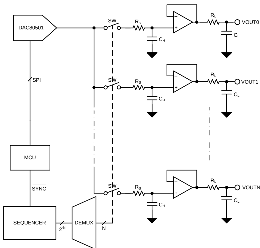
图 15. Multichannel Sample-and-Hold Circuit
