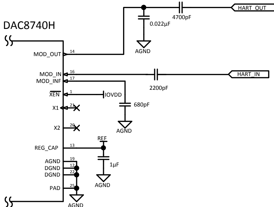
图 33. HART Mode: DAC874xH Passive Selection For Internal Filter
