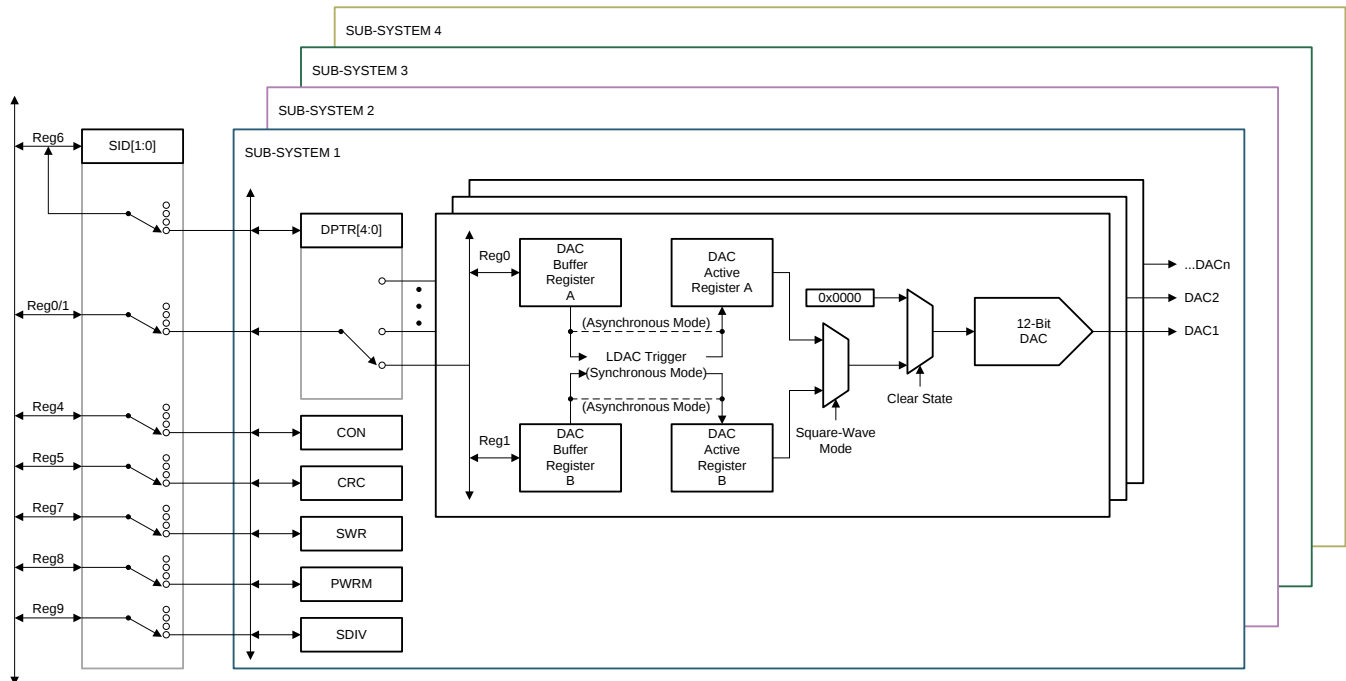
Figure 39. Register Configuration
