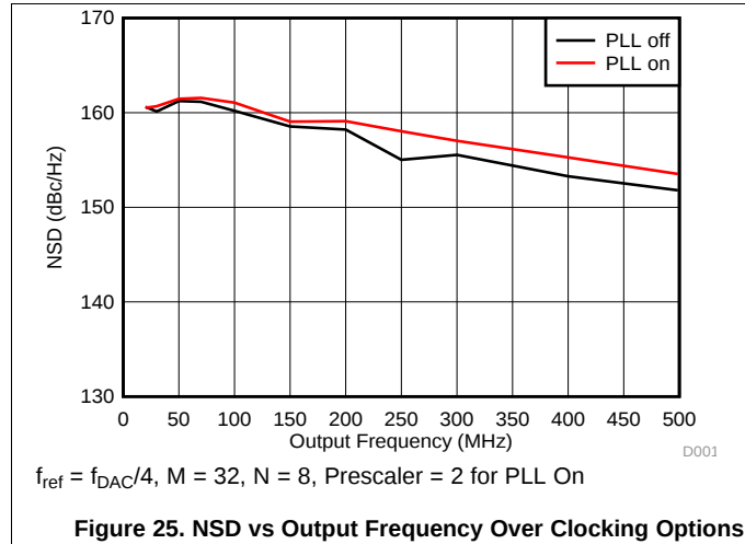
Figure 25. NSD vs Output Frequency Over Clocking Options
