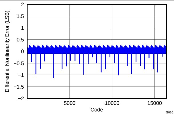
Figure 6. Differential Nonlinearity
