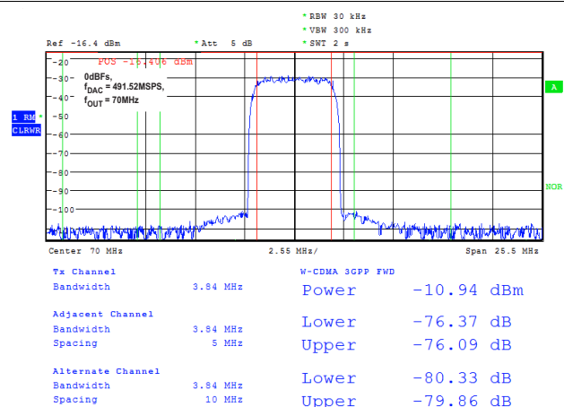
Figure 22. Single-Carrier WCDMA Test Mode 1
