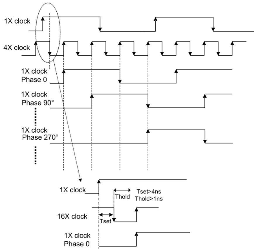
图 72. 8 \times f_{cw} and 4 \times f_{cw} Timing Diagram
