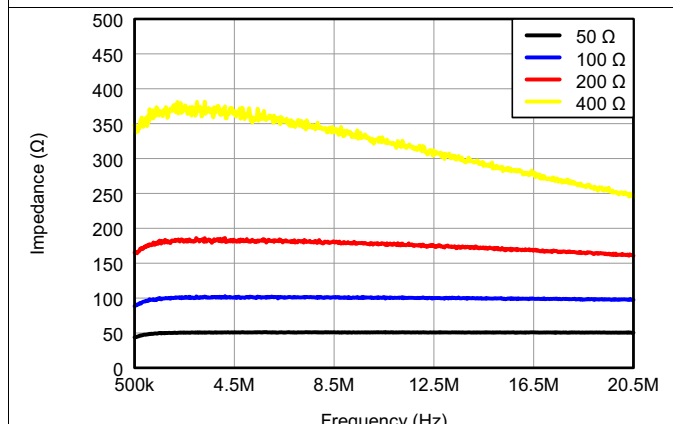
图 10. Input Impedance With Active Termination (Magnitude)
