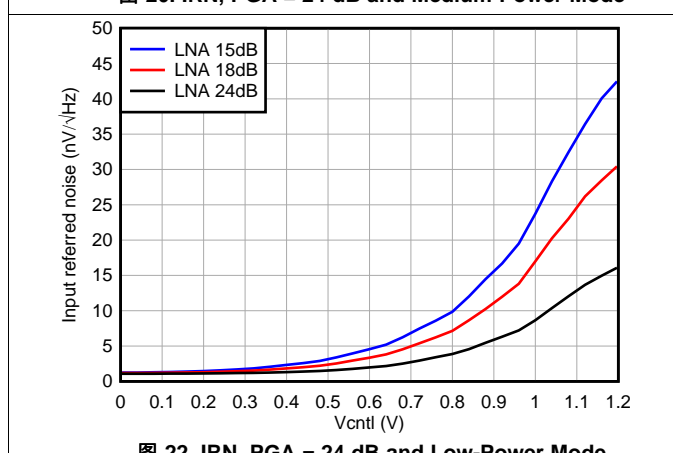
图 22. IRN, PGA = 24 dB and Low-Power Mode
