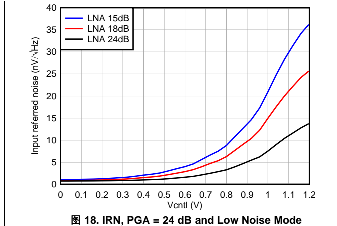
图 18. IRN, PGA = 24 dB and Low Noise Mode
