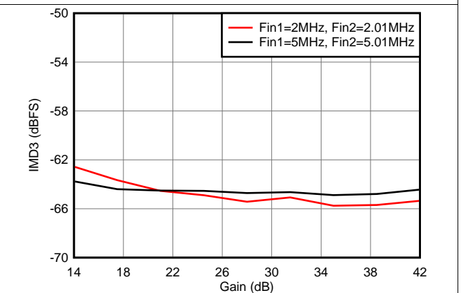
图 45. IMD3, Fout1 = -7 dBFS and Fout2 = -21 dBFS
