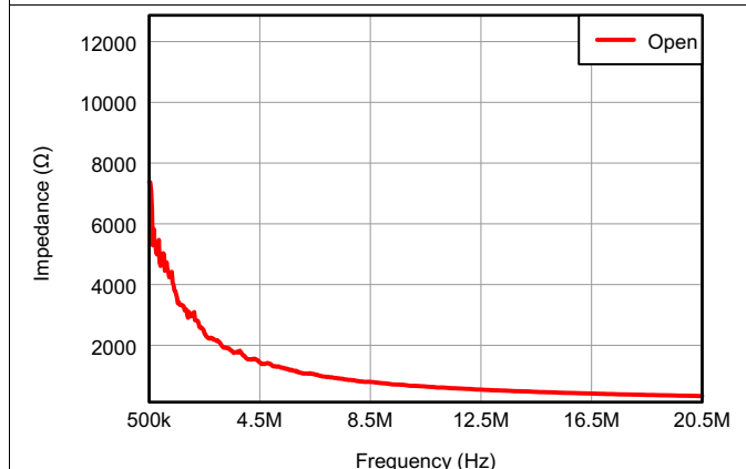
图 8. Input Impedance Without Active Termination (Magnitude)
