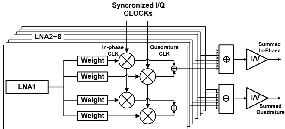
图 73. Block Diagram of 1 \times f_{cw} mode
