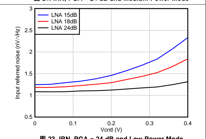
图 23. IRN, PGA = 24 dB and Low-Power Mode
