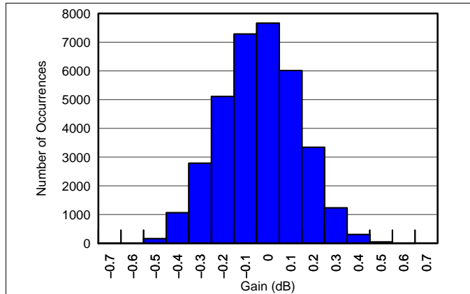
图 6. Gain Matching Histogram, V_{CNTL} = 0.9 V (34951 Channels)
