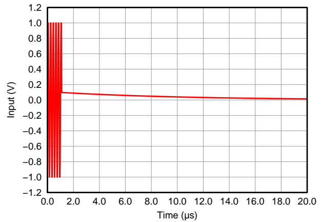
Figure 54. Pulse Inversion Asymmetrical Positive Input
