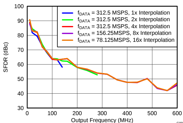
Figure 7. SFDR vs Output Frequency Over Interpolation
