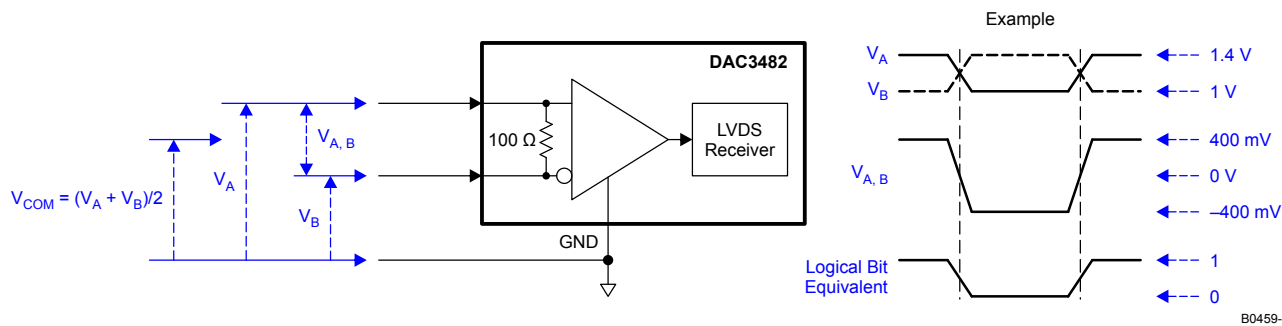
Figure 87. LVDS Data Input Levels
