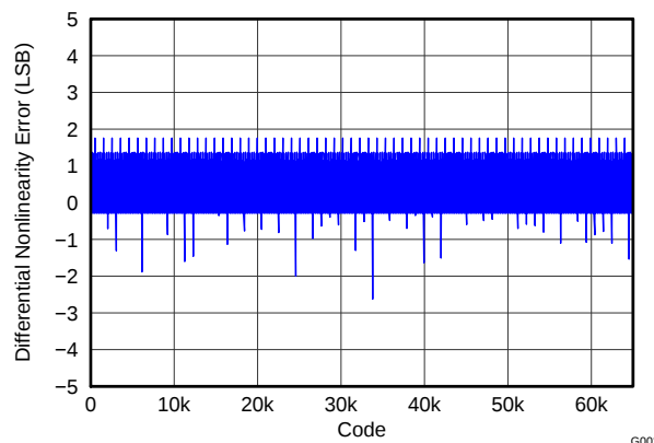
Figure 3. Differential Nonlinearity
