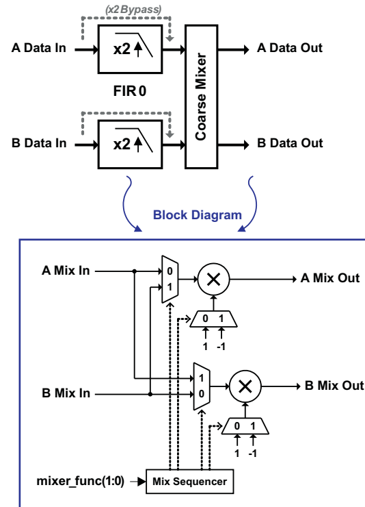
Figure 32. Coarse Mixers Block Diagram
