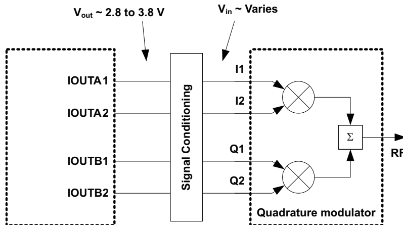
Figure 80. DAC to Analog Quadrature Modulator Interface
