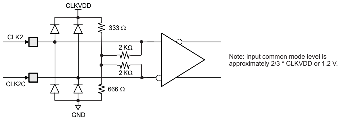
Figure 33. CLK2/C Equivalent Input Circuit
