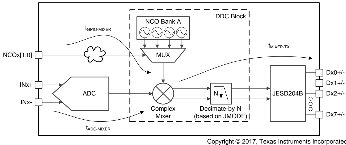
图 68. NCO Fast Frequency Hopping Latency Diagram
