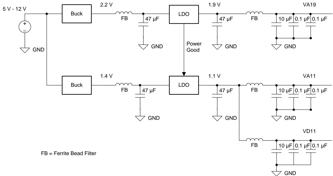
图 184. LDO Linear Regulator Approach Example
