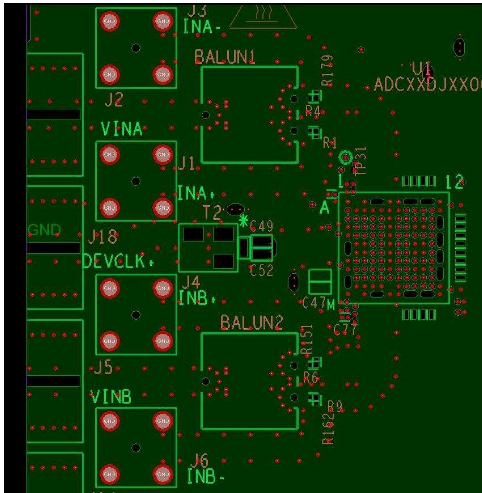
图 187. GND1 Cutouts to Optimize Impedance of Component Pads
