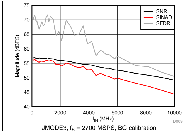
Figure 10. SNR, SINAD, SFDR vs Input Frequency
