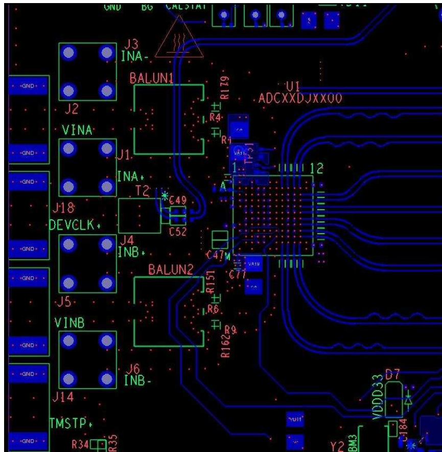
图 188. Bottom Layer Routing: Additional CLK Routing, DA4-7, DB4-7
