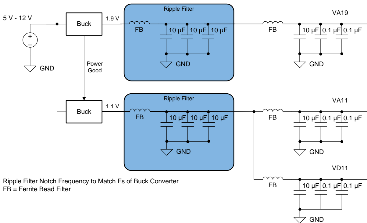
图 185. Switcher-Only Approach Example
