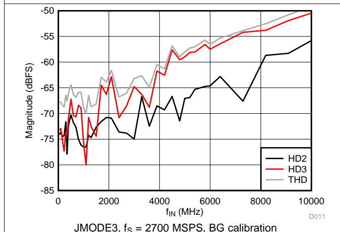
Figure 12. HD2, HD3, THD vs Input Frequency
