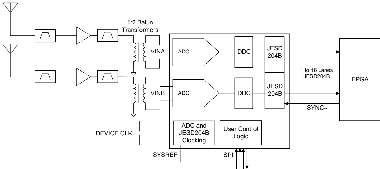
图 180. Typical Configuration for Wideband RF Sampling
