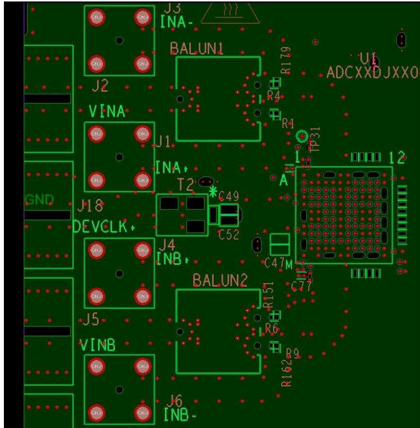
图 186. Top Layer Routing: Analog Inputs, CLK and SYSREF, DA0-3, DB0-3
