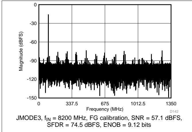
Figure 28. Single-Tone FFT at A_{\text{IN}} = -16\text{ dBFS}
