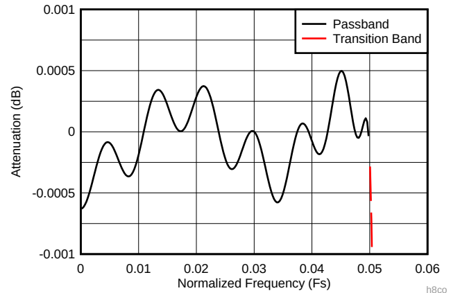
图 79. Decimate-by-8 Composite Zoomed Passband Response
