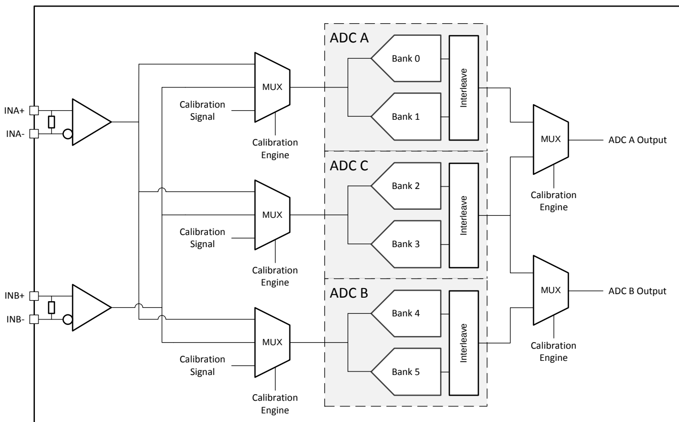
图 86. ADC12DJ3200 Calibration System Block Diagram
