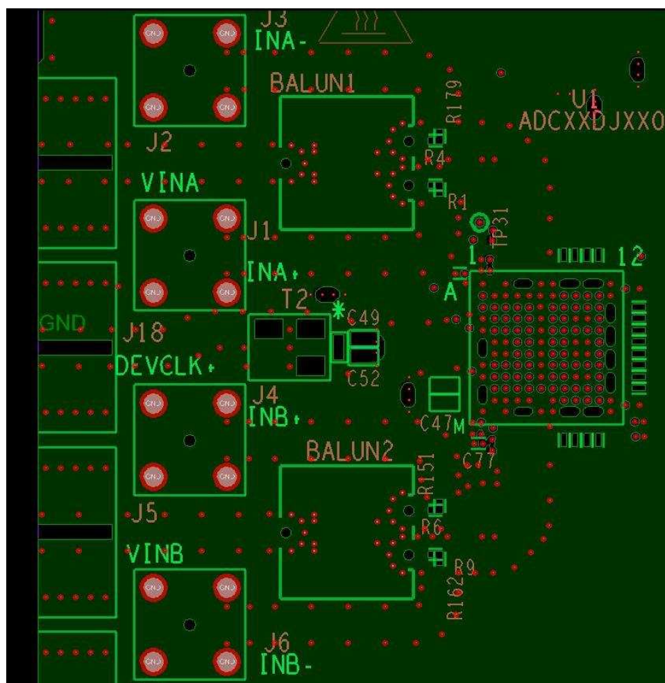
图 188. GND1 Cutouts to Optimize Impedance of Component Pads
