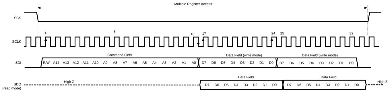
图 88. Serial Interface Protocol - Streaming Read / Write
