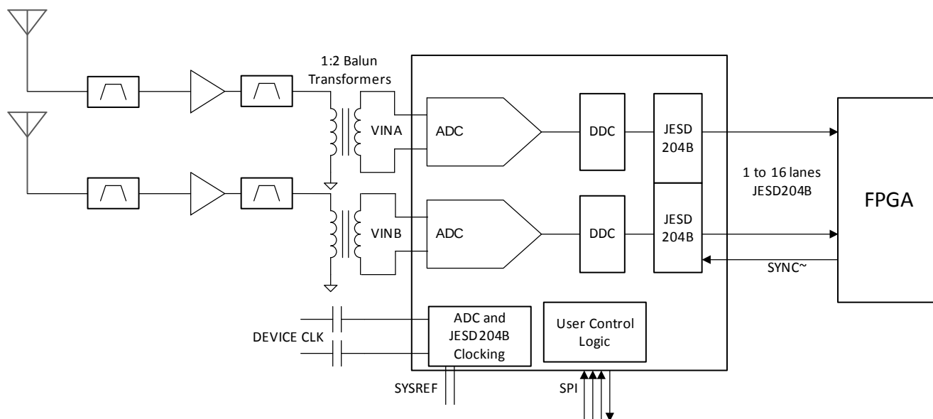
图 181. Typical Configuration for Wideband RF Sampling
