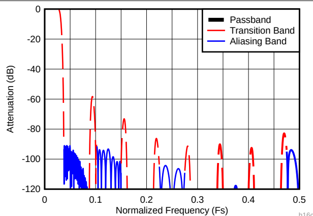
图 80. Decimate-by-16 Composite Response
