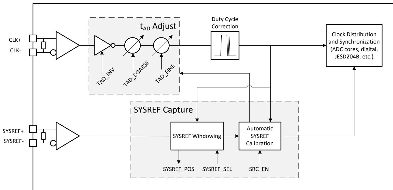
图 66. ADC12DJ3200 Clocking Subsystem
