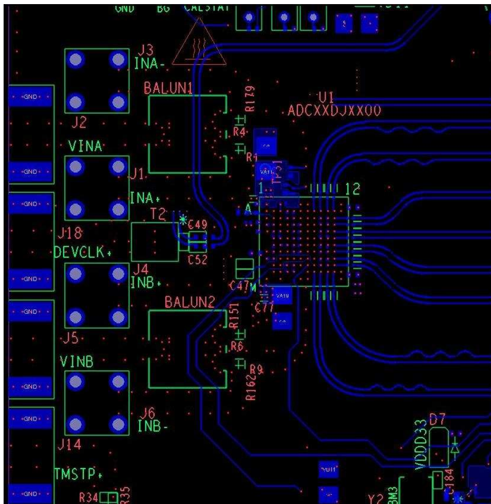
图 189. Bottom Layer Routing - Additional CLK Routing, DA4-7, DB4-7
