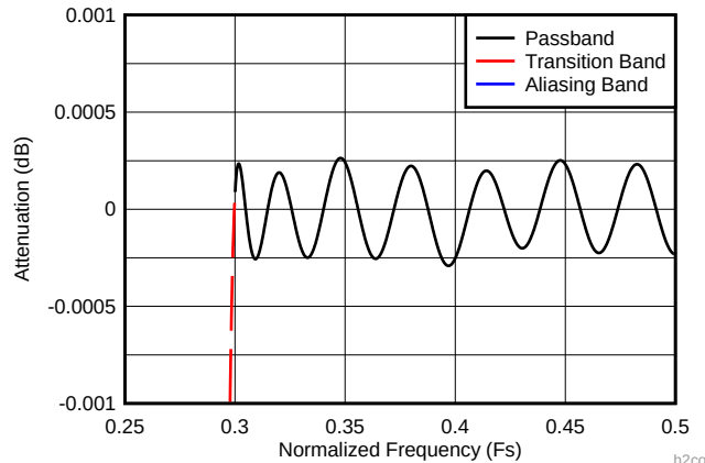
图 73. Decimate-by-2 Composite Zoomed Passband Response (D2_HIGH_PASS = 1)
