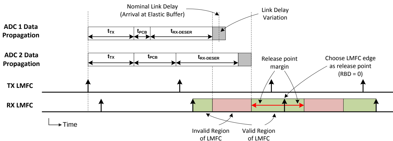
图 83. Definition of valid region of LMFC for elastic buffer release point selection
