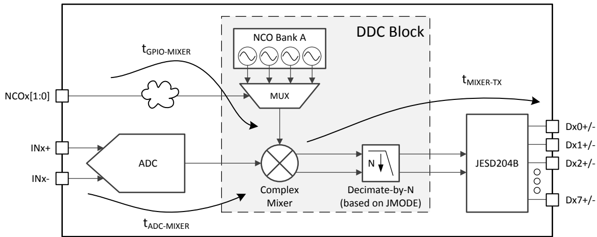
图 69. NCO Fast Frequency Hopping Latency Diagram
