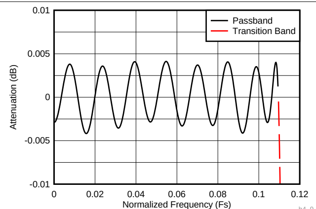
图 77. Decimate-by-4 Composite Zoomed Passband Response (D4_AP87 = 1)
