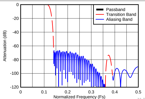
图 76. Decimate-by-4 Composite Response (D4_AP87 = 1)
