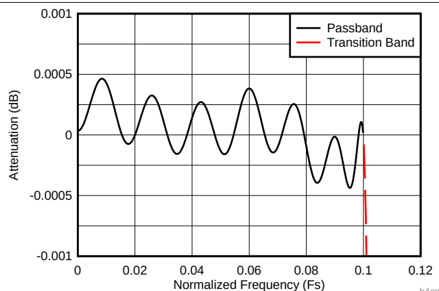
图 75. Decimate-by-4 Composite Zoomed Passband Response (D4_AP87 = 0)
