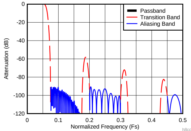
图 78. Decimate-by-8 Composite Response
