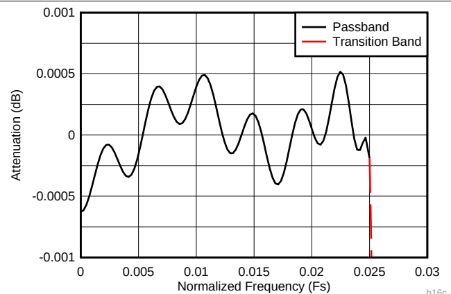
图 81. Decimate-by-16 Composite Zoomed Passband Response
