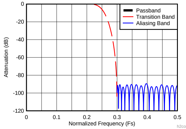
图 9. Decimate-by-2 Composite Response (D2_HIGH_PASS = 0)
