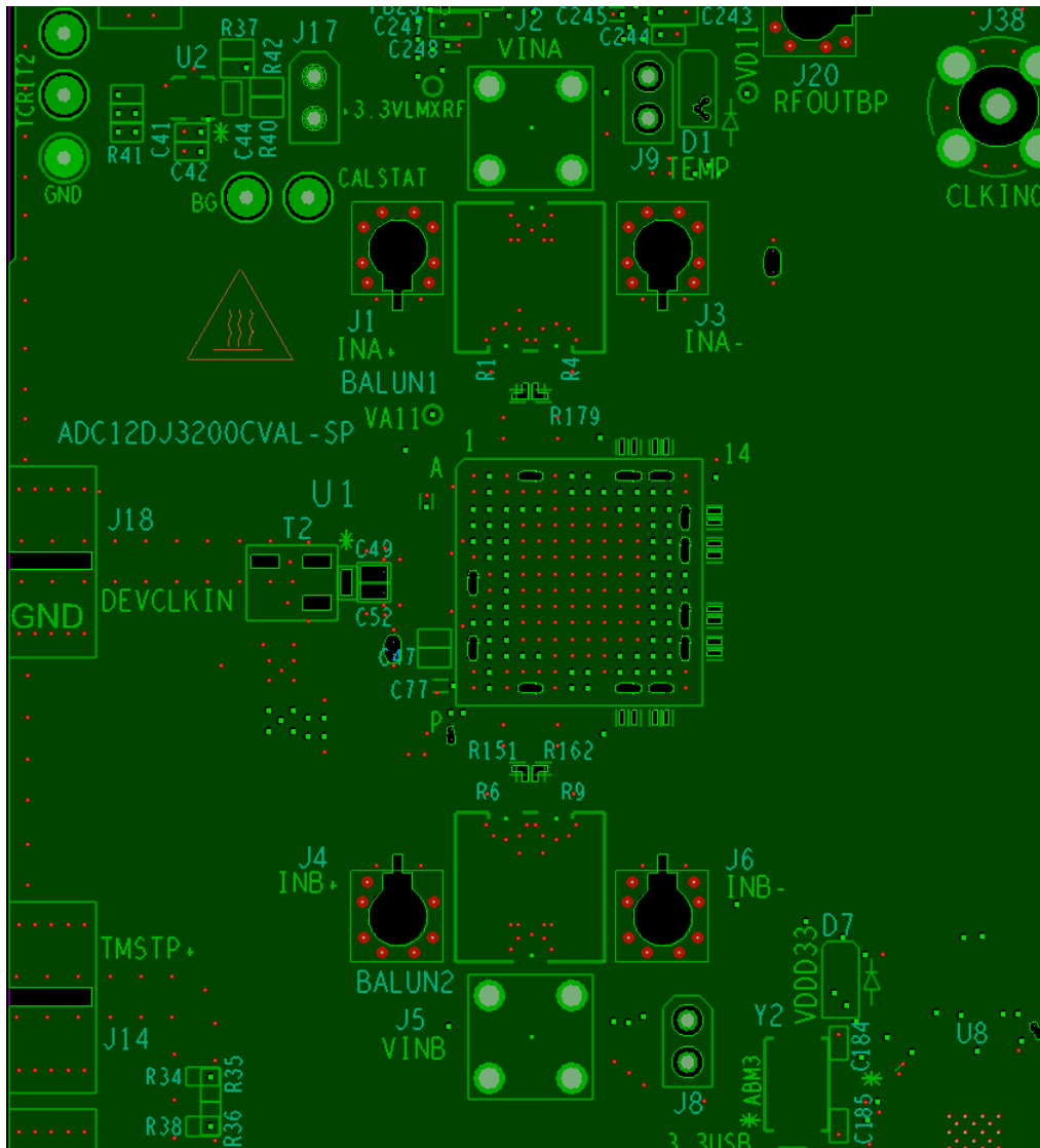
图 124. GND1 Cutouts to Optimize Impedance of Component Pads
