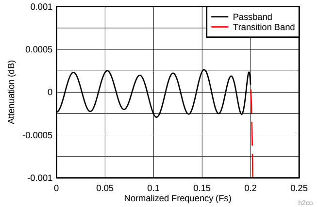
图 10. Decimate-by-2 Composite Zoomed Pass-Band Response (D2_HIGH_PASS = 0)
