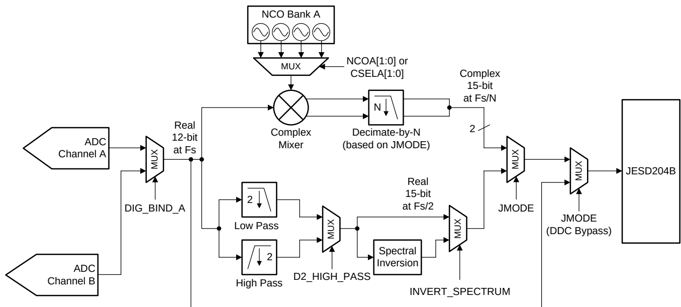
图 7. Channel A Digital Down Conversion Block (Dual-Channel Mode Only)
