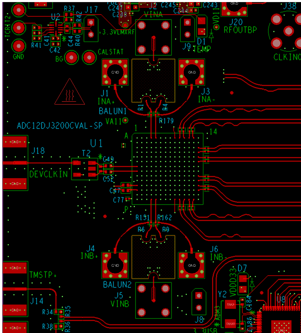
图 123. Top Layer Routing: Analog Inputs, CLK and SYSREF, DA0-3, DB0-3
