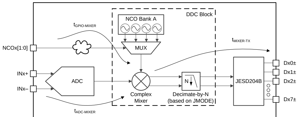
图 8. NCO Fast Frequency Hopping Latency Diagram
