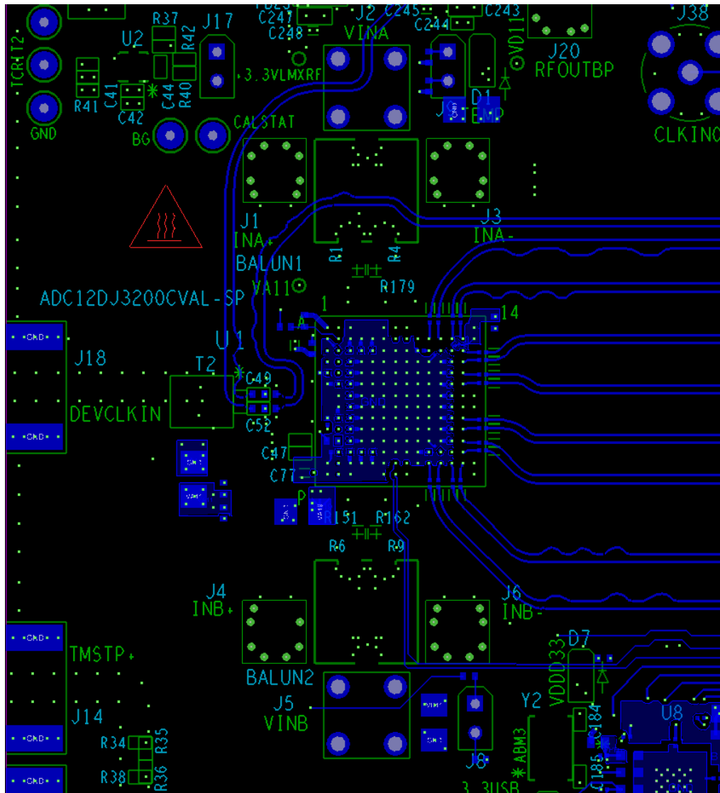
图 125. Bottom Layer Routing: Additional CLK Routing, DA4-7, DB4-7
