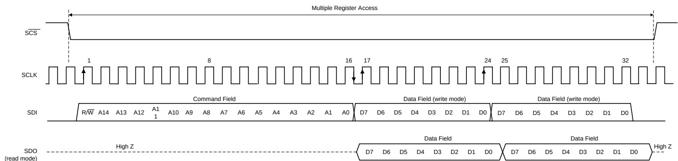
图 27. Serial Interface Protocol: Streaming Read and Write
