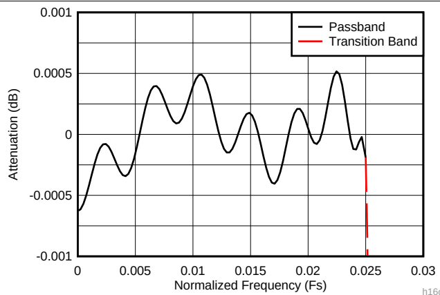
图 18. Decimate-by-8 Composite Zoomed Pass-Band Response
