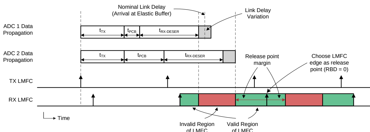
图 22. LMFC Valid Region Definition for Elastic Buffer Release Point Selection
