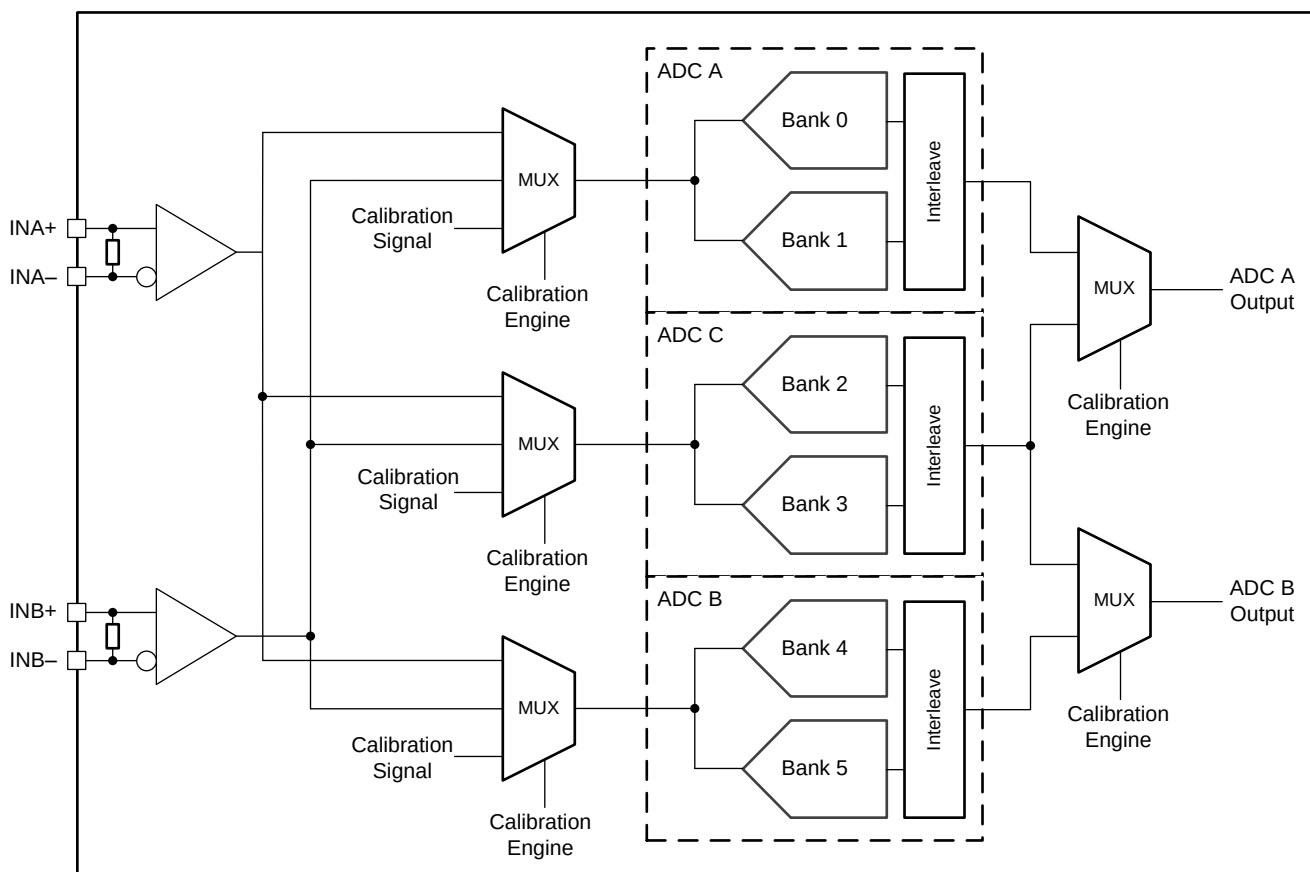
图 25. ADC12DJ3200QML-SP Calibration System Block Diagram
