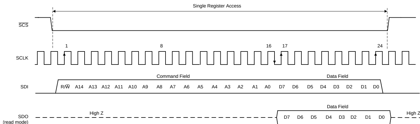
图 26. Serial Interface Protocol: Single Read/Write
