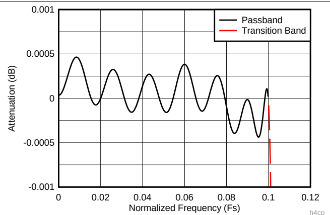
图 12. Decimate-by-2 Composite Zoomed Pass-Band Response (D2_HIGH_PASS = 1)
