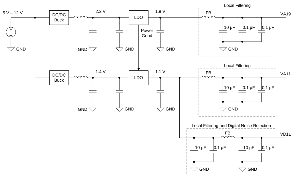
图 121. LDO Linear Regulator Example
