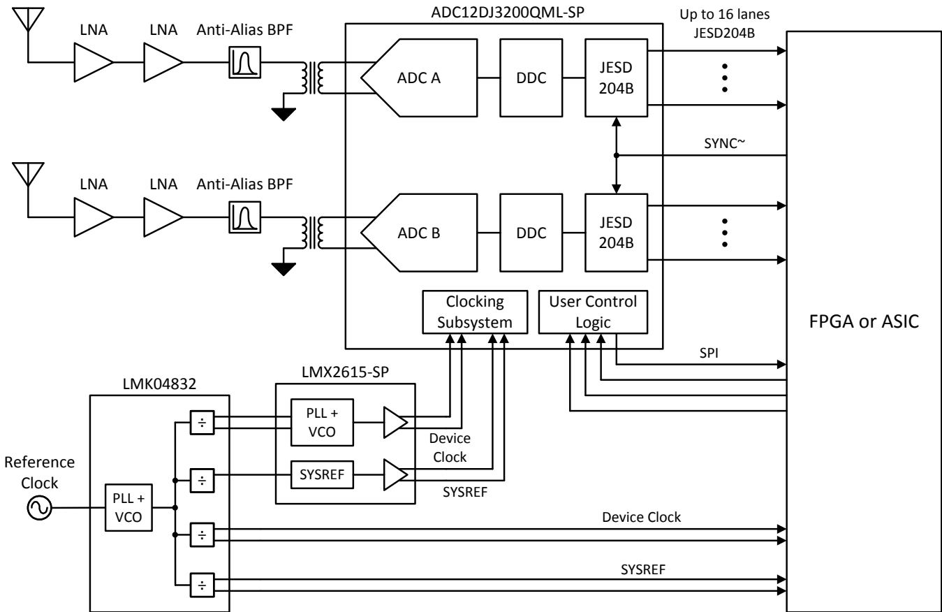
图 120. Typical Configuration for Wideband RF Sampling Receiver
