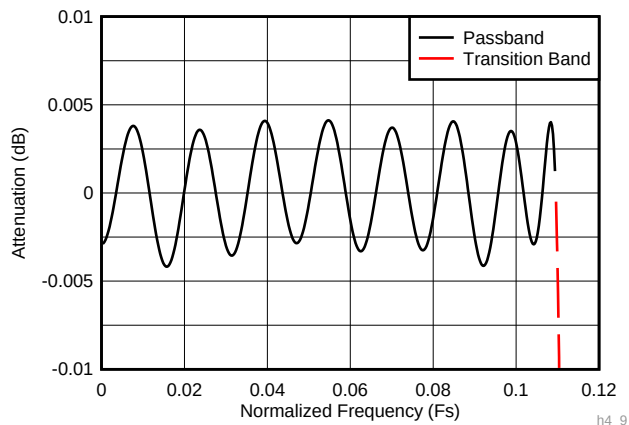
图 16. Decimate-by-4 Composite Zoomed Pass-Band Response (D4_AP87 = 1)
