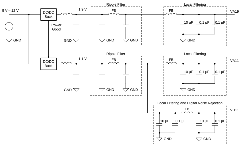
图 122. DC/DC Switching Regulator Example
