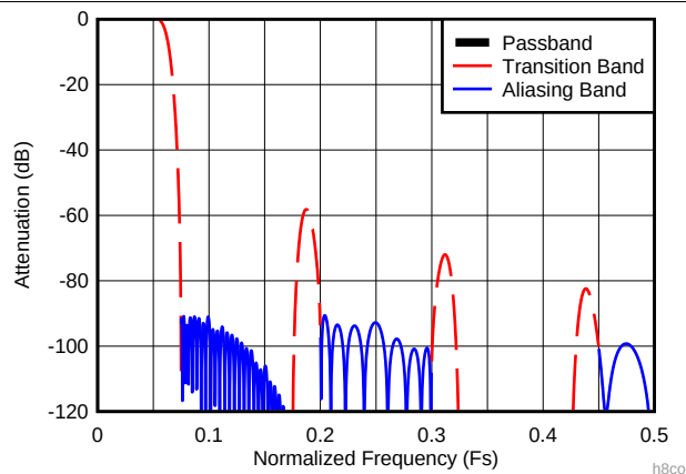
图 15. Decimate-by-4 Composite Response (D4_AP87 = 1)
