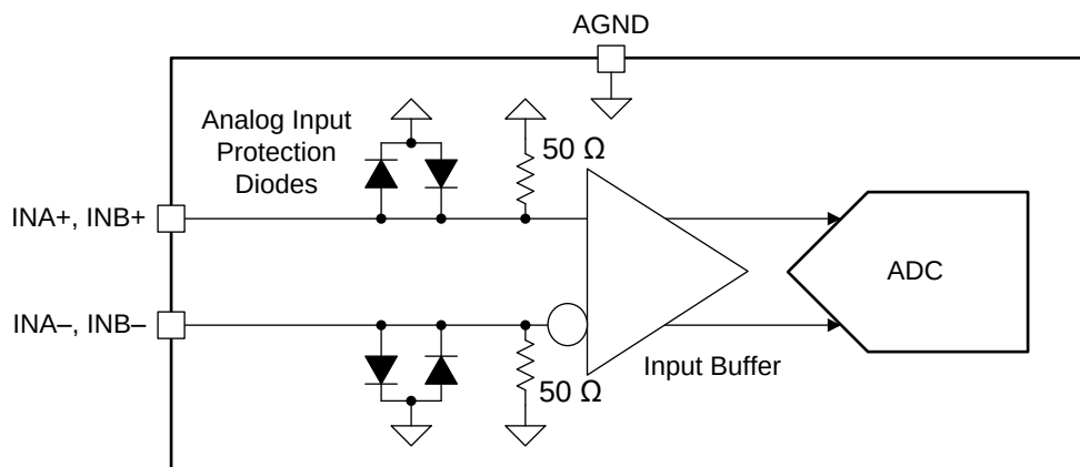
图 4. ADC12DJ3200QML-SP Analog Input Internal Termination and Protection Diagram
