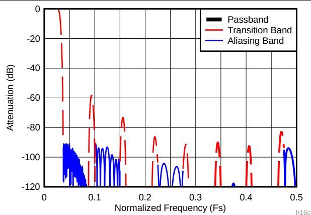
图 19. Decimate-by-16 Composite Response
