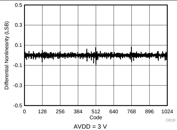
Figure 17. Typical DNL
