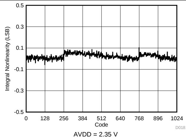
Figure 16. Typical INL
