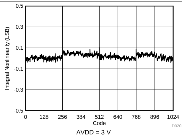
Figure 18. Typical INL
