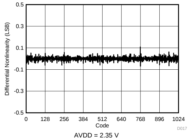
Figure 15. Typical DNL
