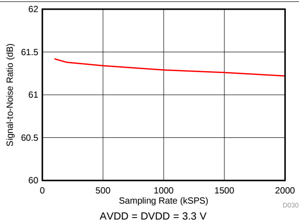
Figure 27. SNR vs Sampling Rate
