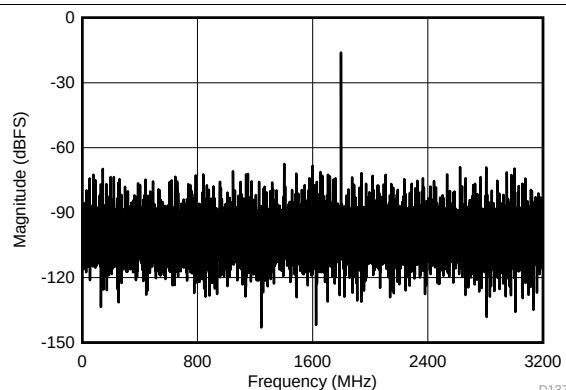
JMODE5, f_{\text{IN}} = 8200\text{ MHz} , FG calibration, SNR = 49.0 dBFS, SFDR = 67.5 dBFS, ENOB = 7.79 bits
