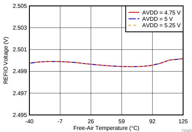
60. Variation of Internal Reference Output (REFIN/REFOUT) vs Free-Air Temperature and Supply
