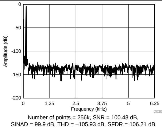
图 34. Typical FFT Plot for OSR 16x (±10 V)
