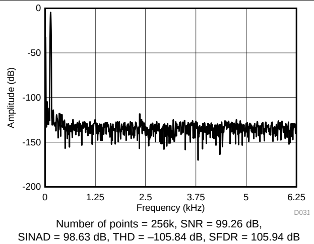
图 35. Typical FFT Plot for OSR 16x (±5 V)
