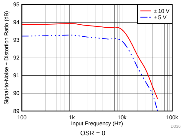
图 40. SINAD vs Input Frequency for Different Input Ranges
