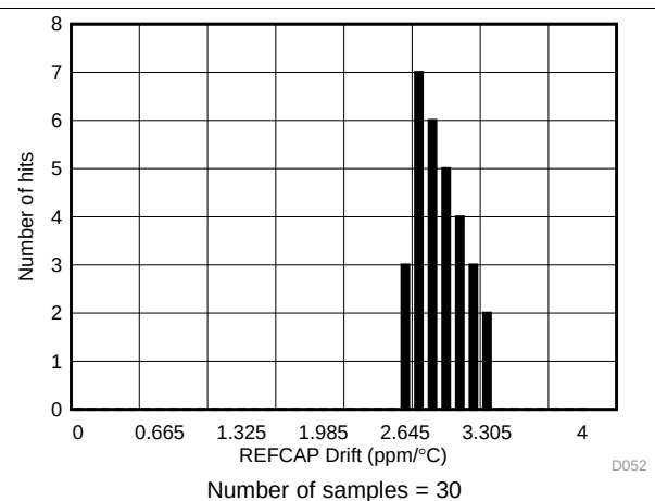
图 63. Reference Buffer Temperature Drift Histogram
