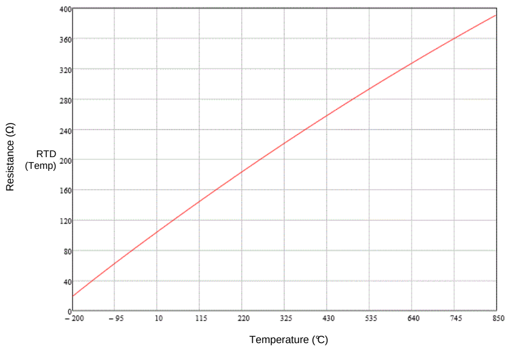
Figure 77. PT-100 RTD Resistance from –200°C to 850°C
