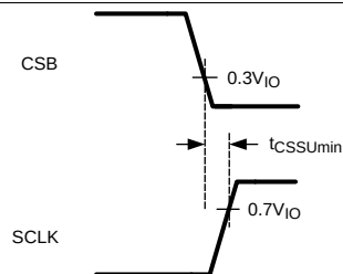
Figure 2. CBS Setup Time
