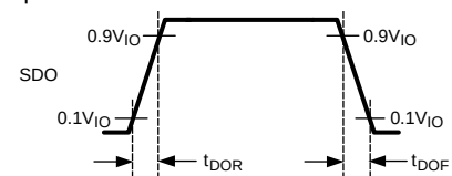
Figure 7. SDO Rise and Fall Time
