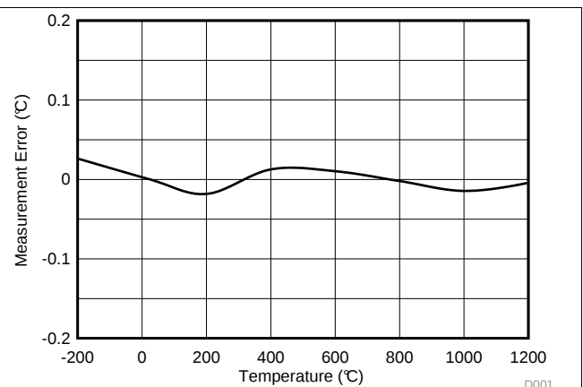
图 73. Temperature Measurement Error vs T_{(TC)}
