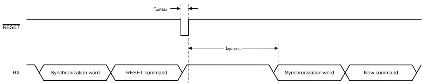
图 2. RESET Pin and RESET Command Timing Requirements
