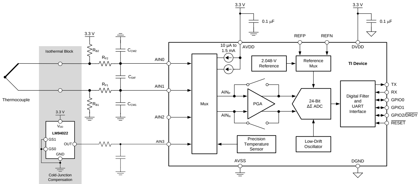
图 76. Thermocouple Measurement
