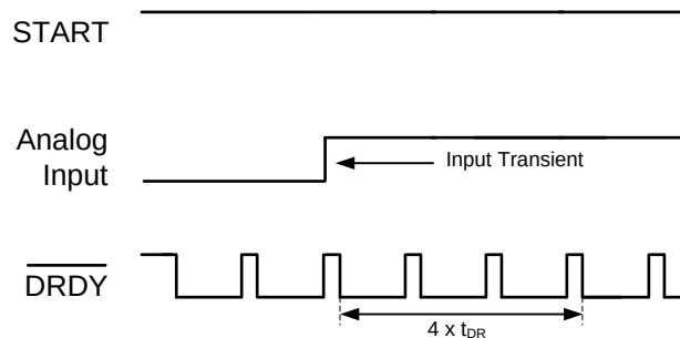
Figure 33. Settling Time for the Input Transient
