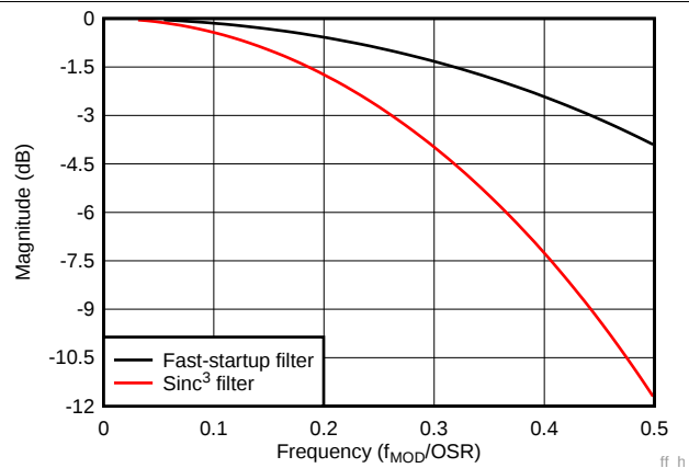
图 10. Fast-Settling and Sinc 3 Digital Filter Response, Pass-Band Detail
