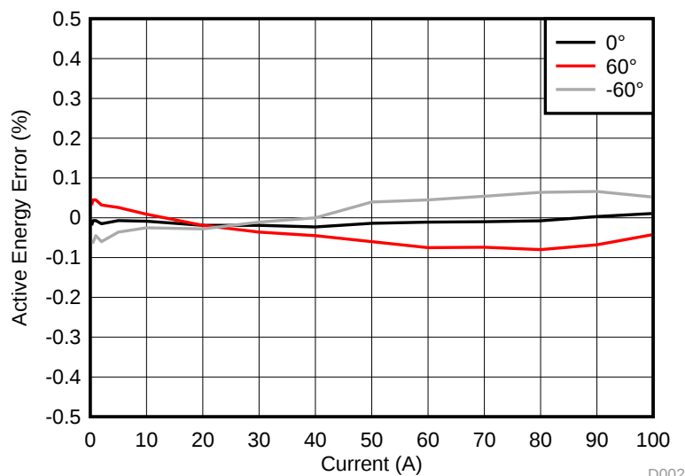
图 50. Phase B Active Energy % Error Versus Current
