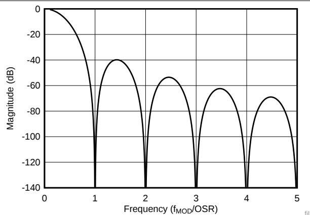
图 6. Sinc 3 Digital Filter Response
