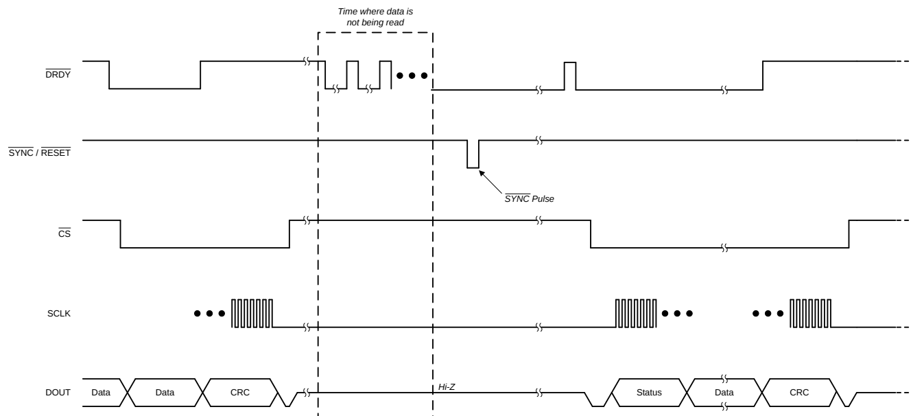
图 20. Collecting Data After a Hiatus Using the \overline{\text{SYNC}}/\overline{\text{RESET}} Pin
