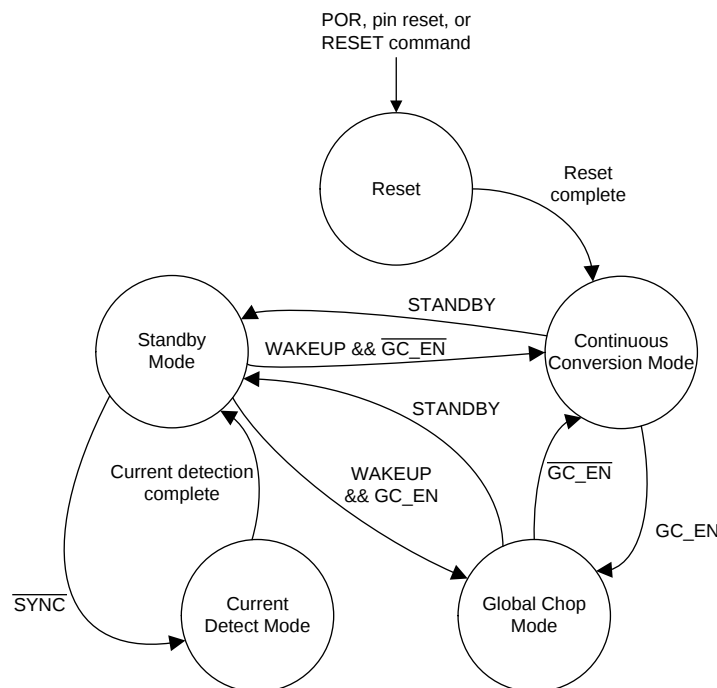
图 16. State Diagram Depicting Device Functional Modes
