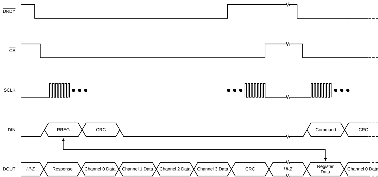
图 22. Reading a Single Register
