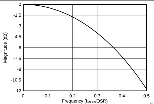
图 7. Sinc 3 Digital Filter Response, Pass-Band Detail
