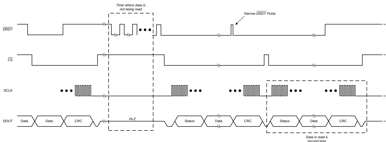
图 21. Collecting Data After a Hiatus by Reading Data Twice
