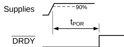
图 3. Power-On-Reset Timing
