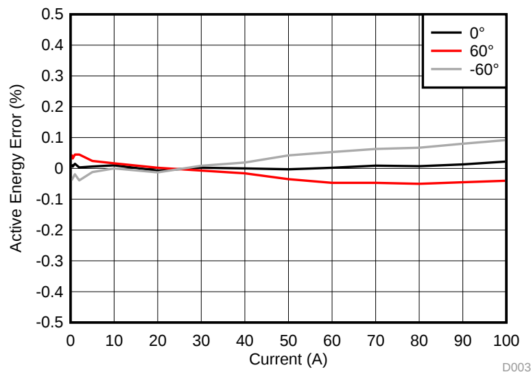
图 51. Cumulative Phase Active Energy % Error Versus Current
