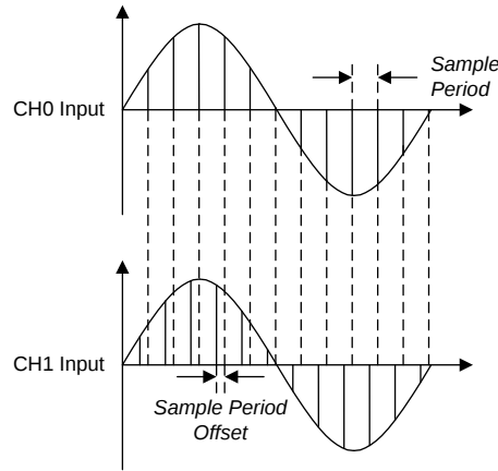
图 13. Channel 1 With a Positive Sample Phase Shift With Respect to Channel 0
