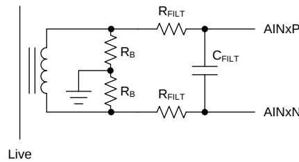
图 48. Current Measurement Front-End
