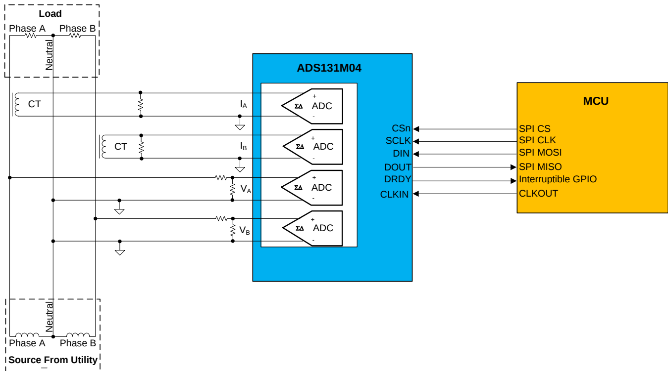
图 46. Split-Phase Metrology Design Front-End
