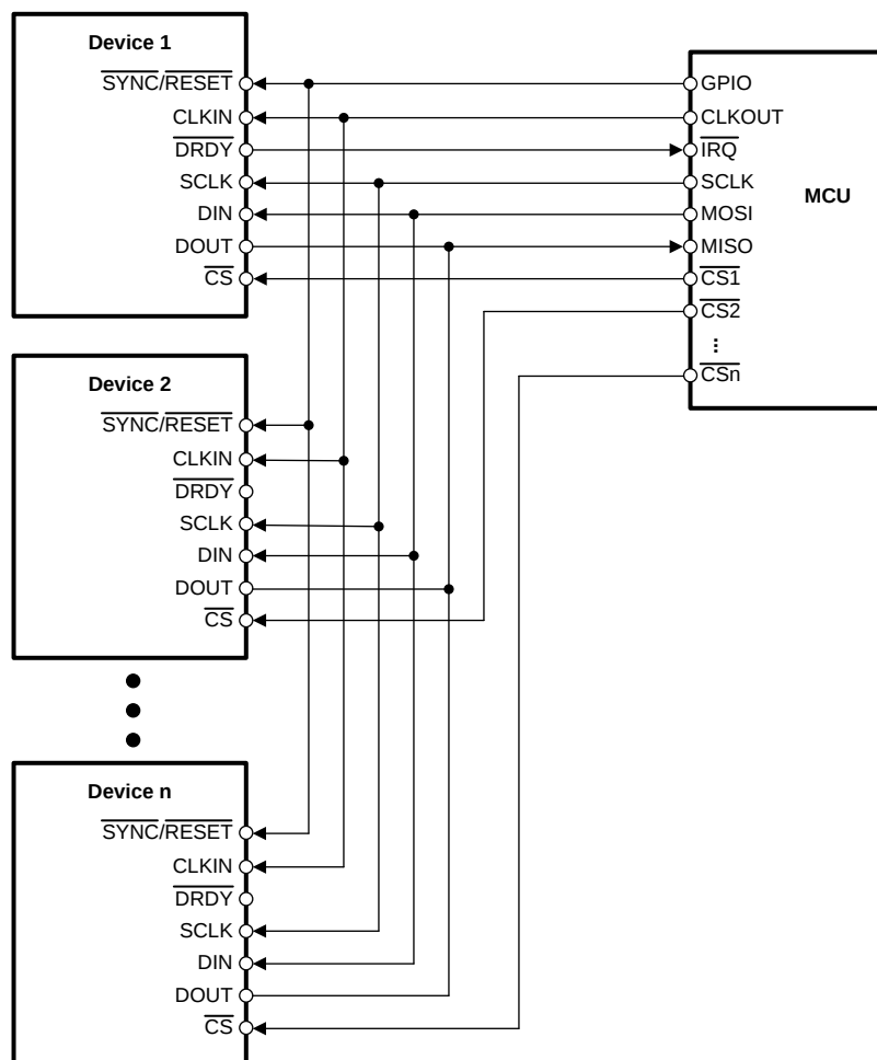
图 45. Multiple Device Configuration
