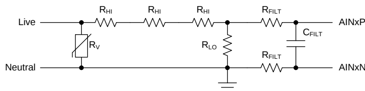
图 47. Voltage Measurement Front-End
