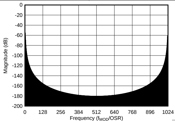
图 8. Sinc 3 Digital Filter Response, OSR 1024, Stop-Band Detail
