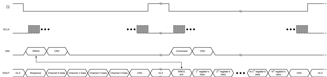
图 23. Reading Multiple Registers
