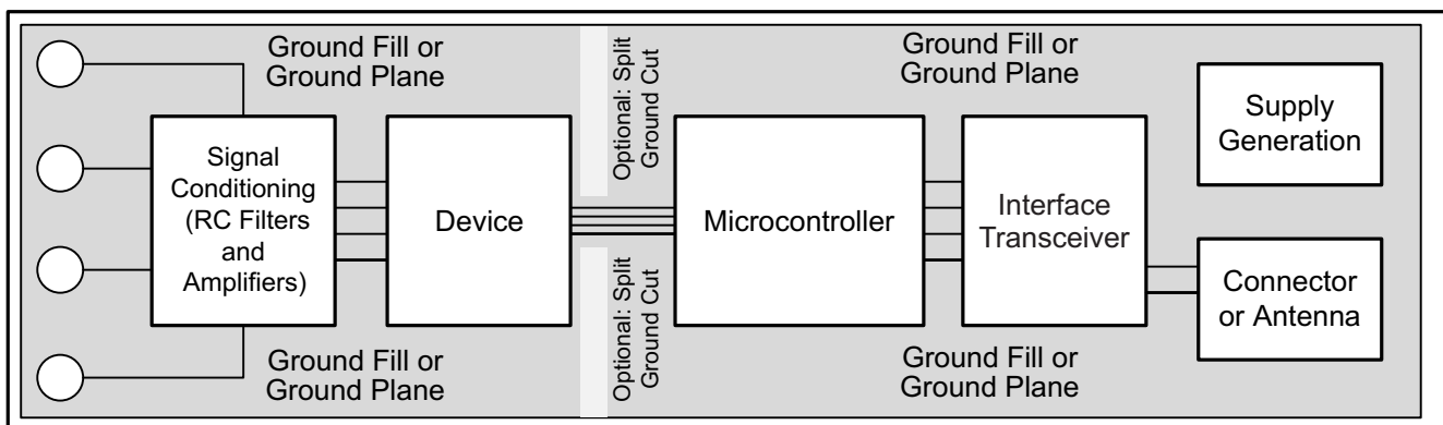
图 57. System Component Placement
