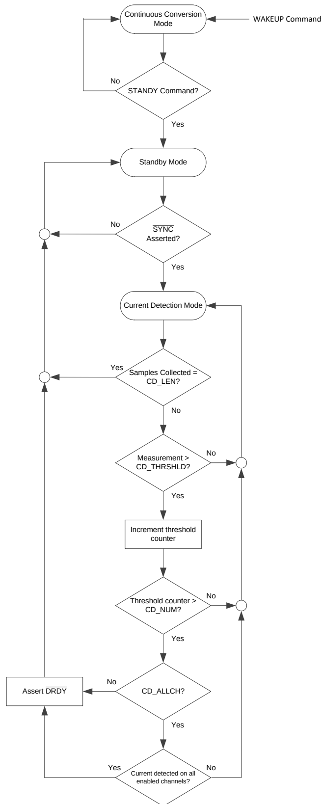
图 17. Current Detect Mode Flow Chart
