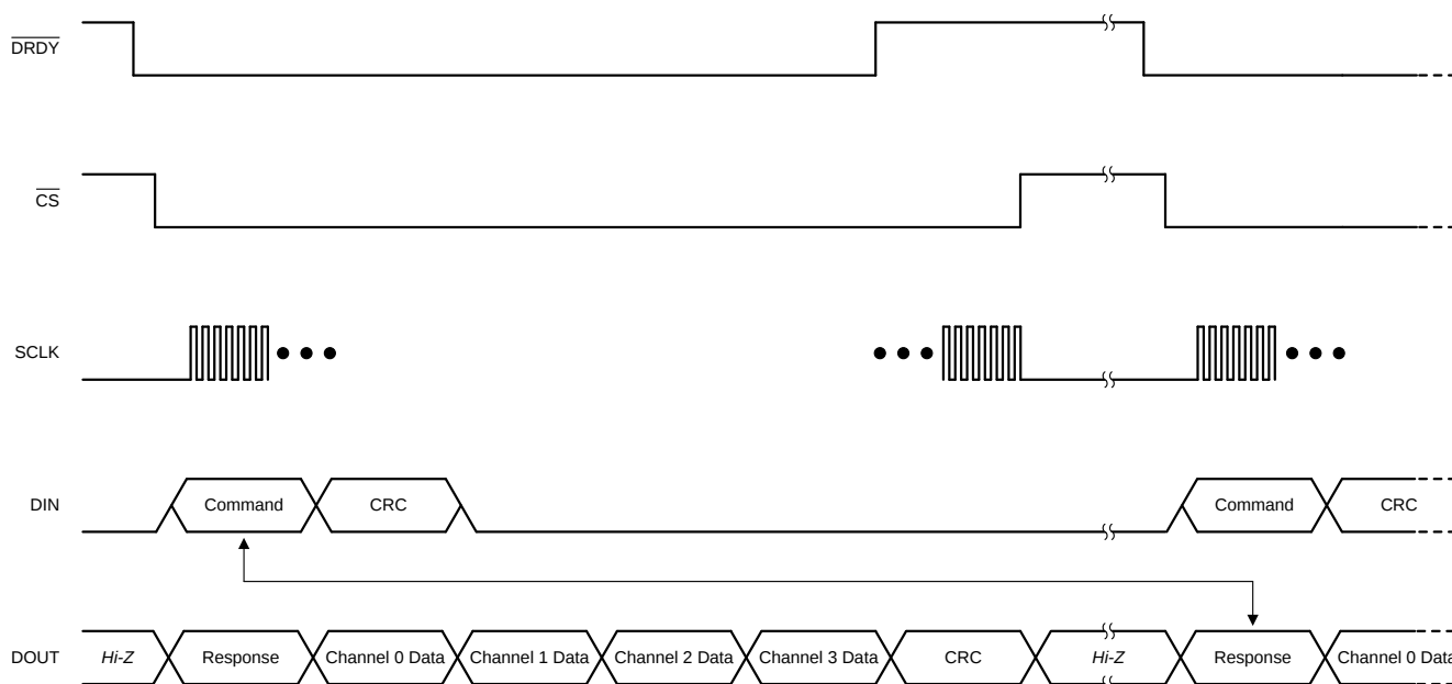
图 18. Typical Communication Frame
