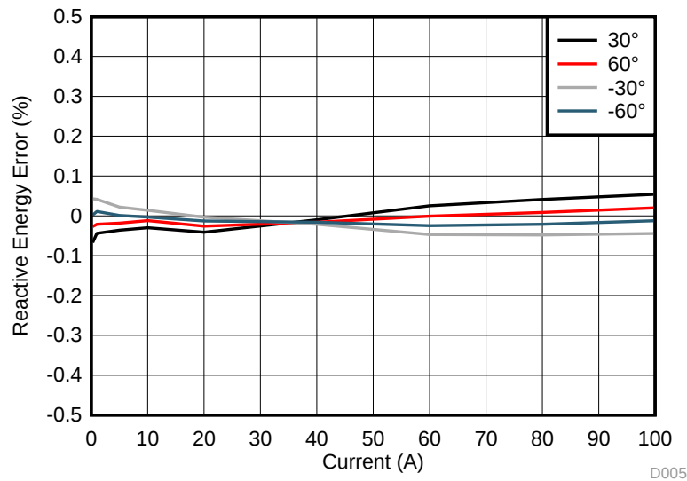
图 52. Cumulative Reactive Energy % Error Versus Current
