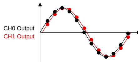
图 14. Channels 1 and 0 From the Perspective of the Host
