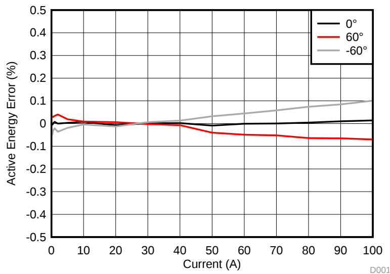
图 49. Phase A Active Energy % Error Versus Current
