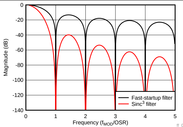
图 9. Fast-Settling and Sinc 3 Digital Filter Response
