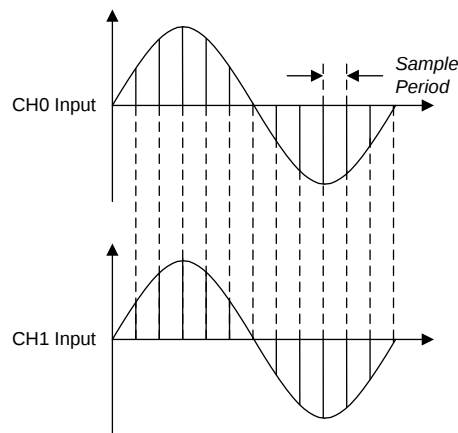
图 12. Two Channel Outputs With Equal Phase Settings
