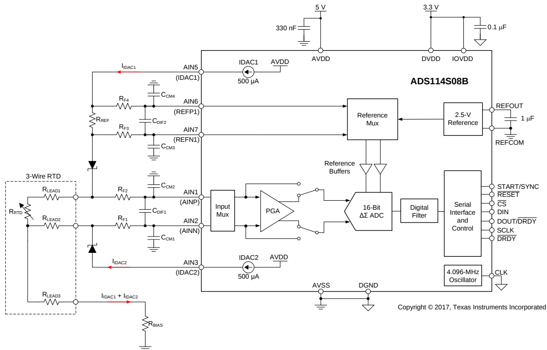
图 96. 3-Wire RTD Application
