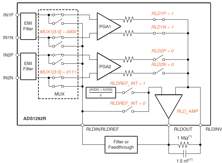
Figure 47. Example RLDOOUT Signal Configured to be Routed to IN2N
