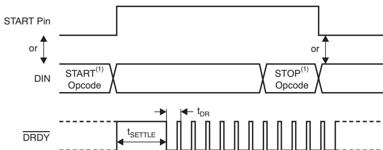
Figure 38. Continuous Conversion Mode
