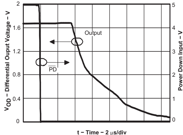
Figure 30. Turnoff Time
