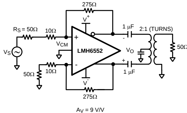
Figure 48. Noise Figure Circuit Configuration
