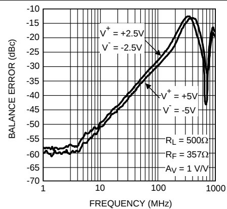
Figure 30. Balance Error
