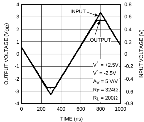
Figure 26. Overdrive Recovery
