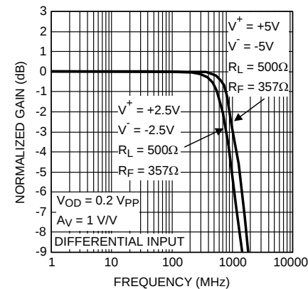
Figure 5. Frequency Response vs Supply Voltage
