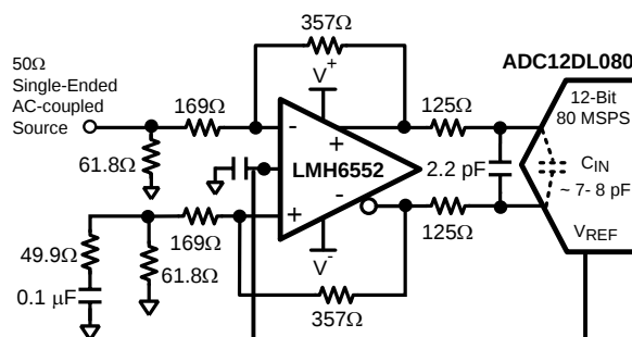
Figure 47. Split Supply
