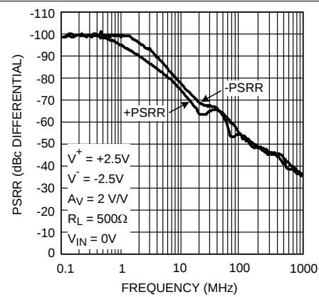
Figure 28. PSRR
