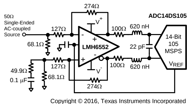
Figure 51. Driving a 14-bit ADC
