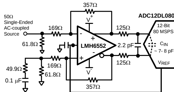
Figure 49. Driving a 12-Bit ADC
