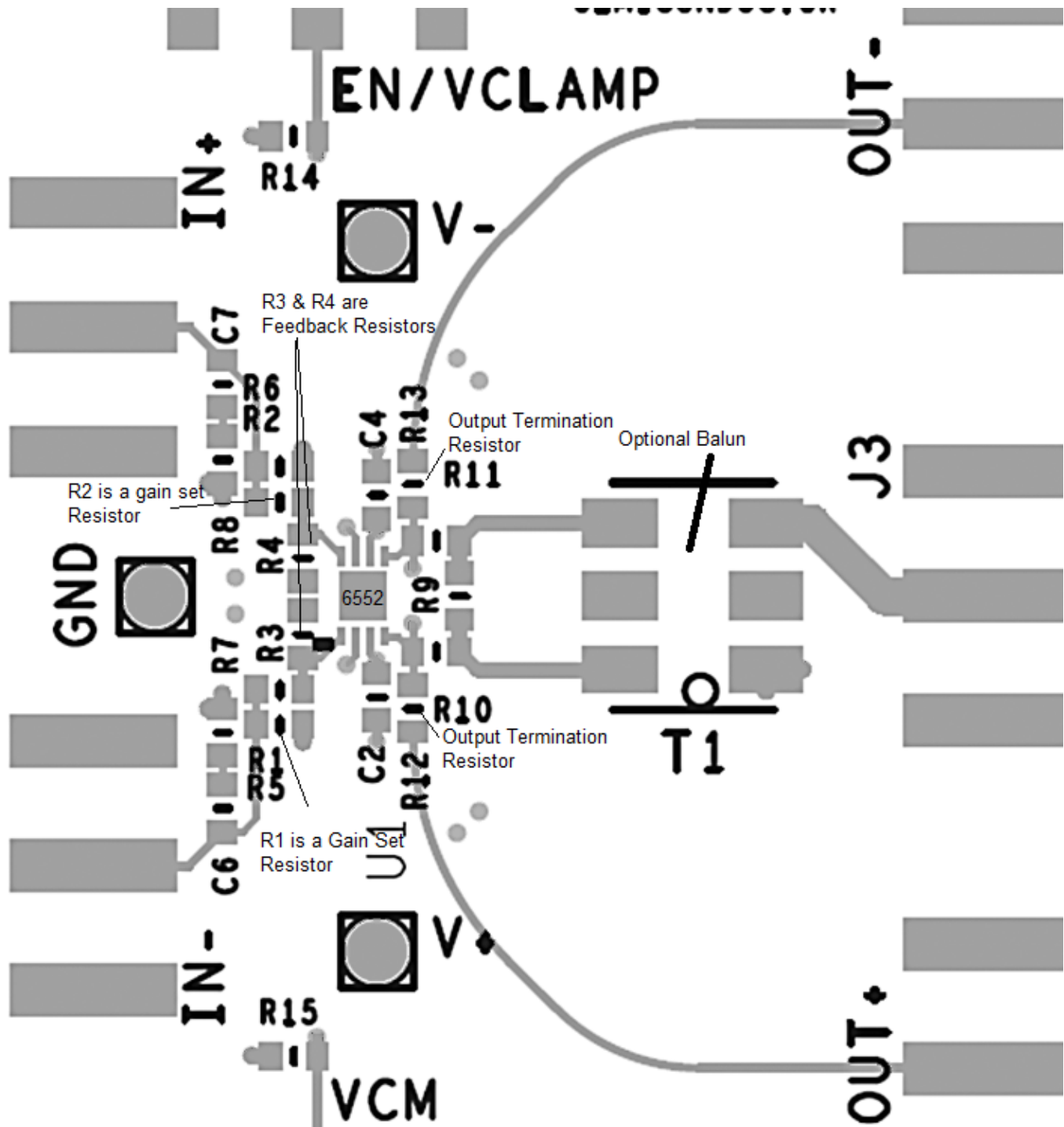
Figure 55. Layout Schematic
