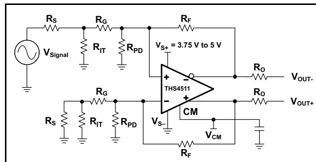
Figure 46. THS4511 DC-Coupled Single-Source Supply Range From 3.75 V to 5 V With R_{PD} Used To Set V_{IC}
