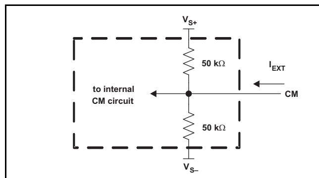
Figure 45. CM Input Circuit
