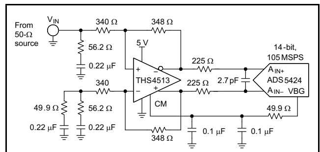
Figure 86. THS4513 and ADS5424 Circuit
