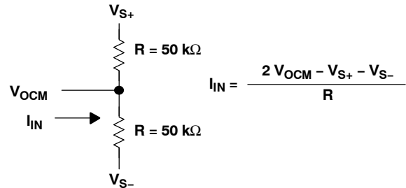
Equivalent Input Circuit for V_{OCM} Figure 102
