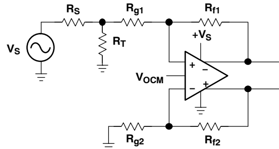
Application Circuit for the THS4500 and THS4501, Featuring Single-Supply Operation With a Ground-Referenced Input Signal
