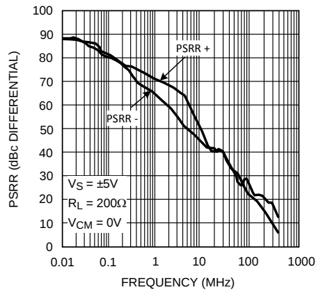
Figure 19. PSRR
