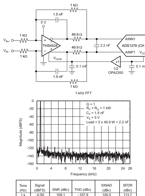
THS4524 and ADS1278 Combined Performance
