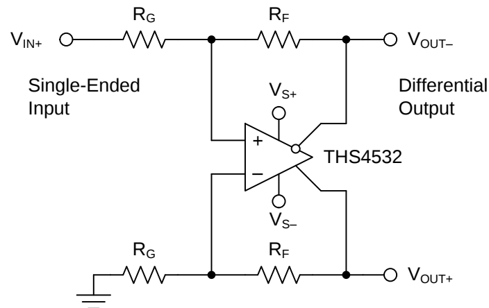
图 97. Single-Ended Input to Differential Output Amplifier
