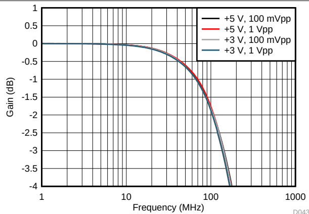
Figure 43. Common-Mode, Small- and Large-Signal Response ( V_{ocm} pin driven)
