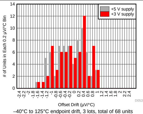
Figure 53. Input Offset Voltage Drift
