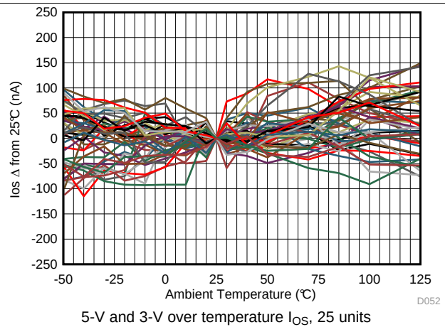
Figure 52. Input Offset Current Over Temperature
