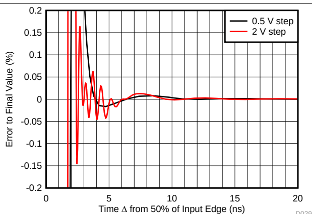
Figure 27. Small- and Large-Signal Step Response
