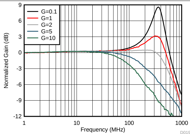
Figure 19. Small-Signal Frequency Response vs Gain
