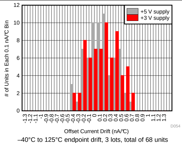
Figure 54. Input Offset Current Drift
