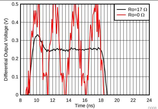
Figure 8. Step Response into Capacitive Load
