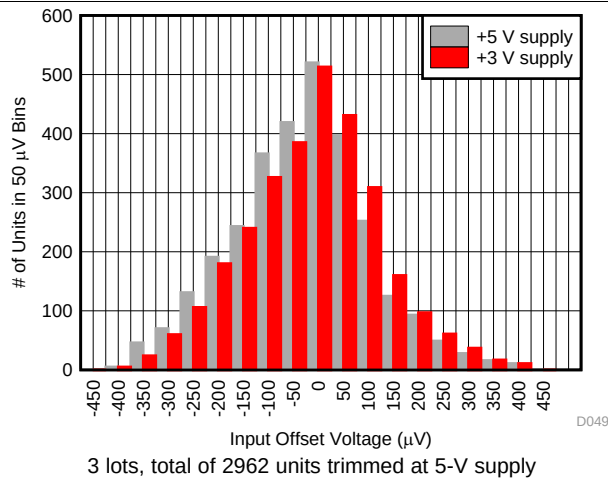
Figure 49. Input Offset Voltage
