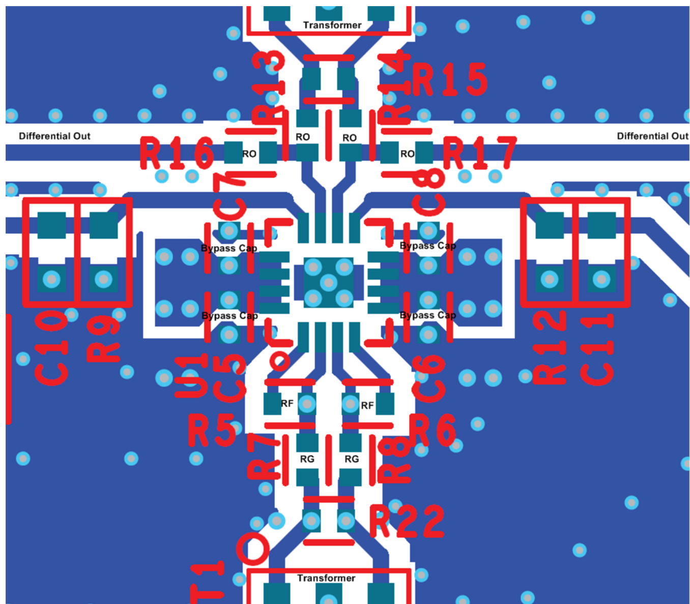
Figure 82. Layout Example
