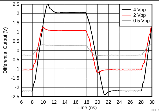
Figure 7. Small and Large Signal Step Response
