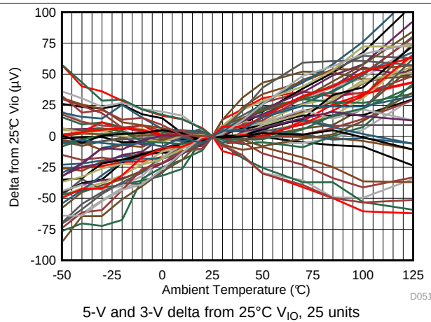
Figure 51. Input Offset Voltage Over Temperature
