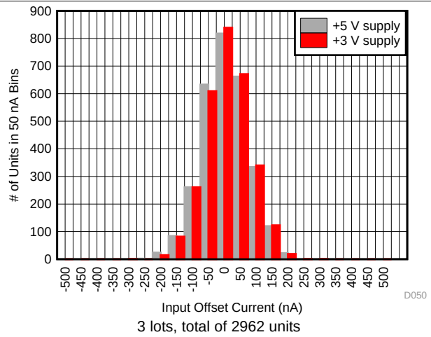
Figure 50. Input offset Current
