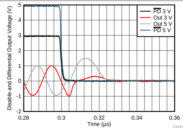
Figure 60. \overline{\text{PD}} Turn Off Waveform
