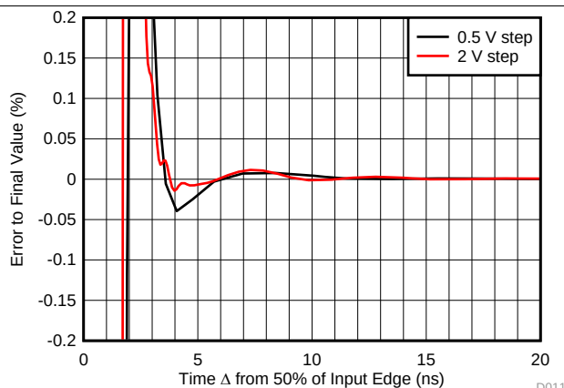
Figure 9. Small- and Large-Signal Step Response
