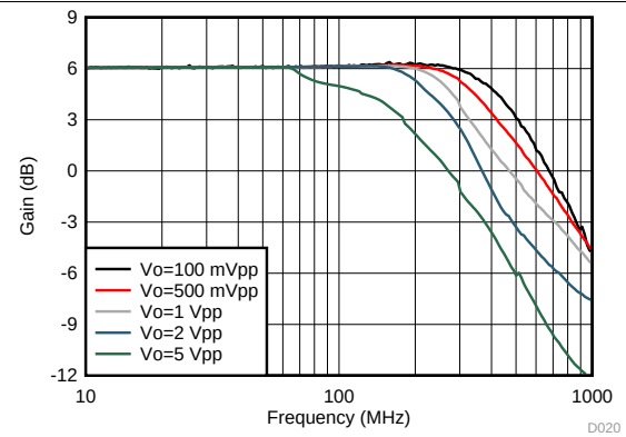
Figure 20. Frequency Response vs V_{opp}
