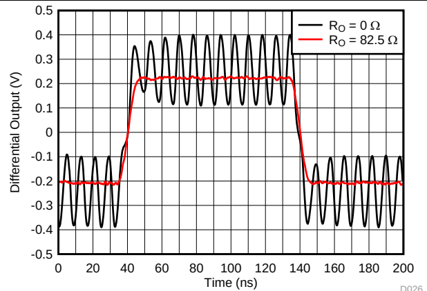
Figure 26. Step Response Into Capacitive Load
