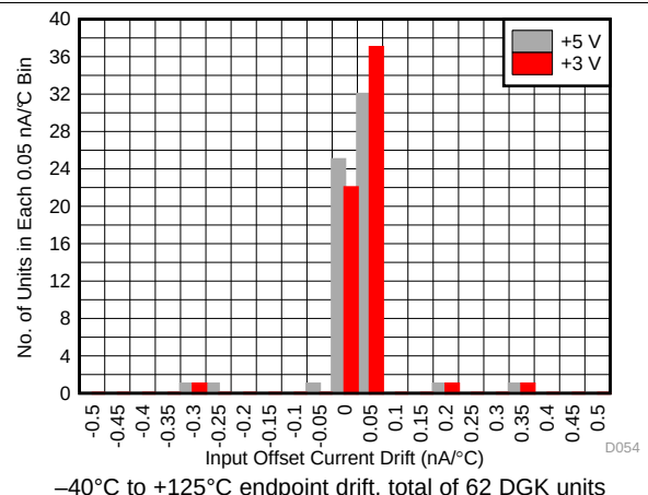
Figure 54. Input Offset Current Drift Histogram
