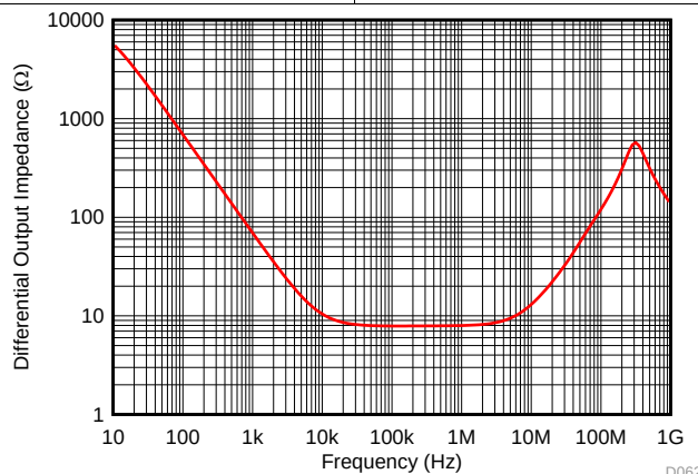
Figure 68. Differential Open-Loop Output Impedance
