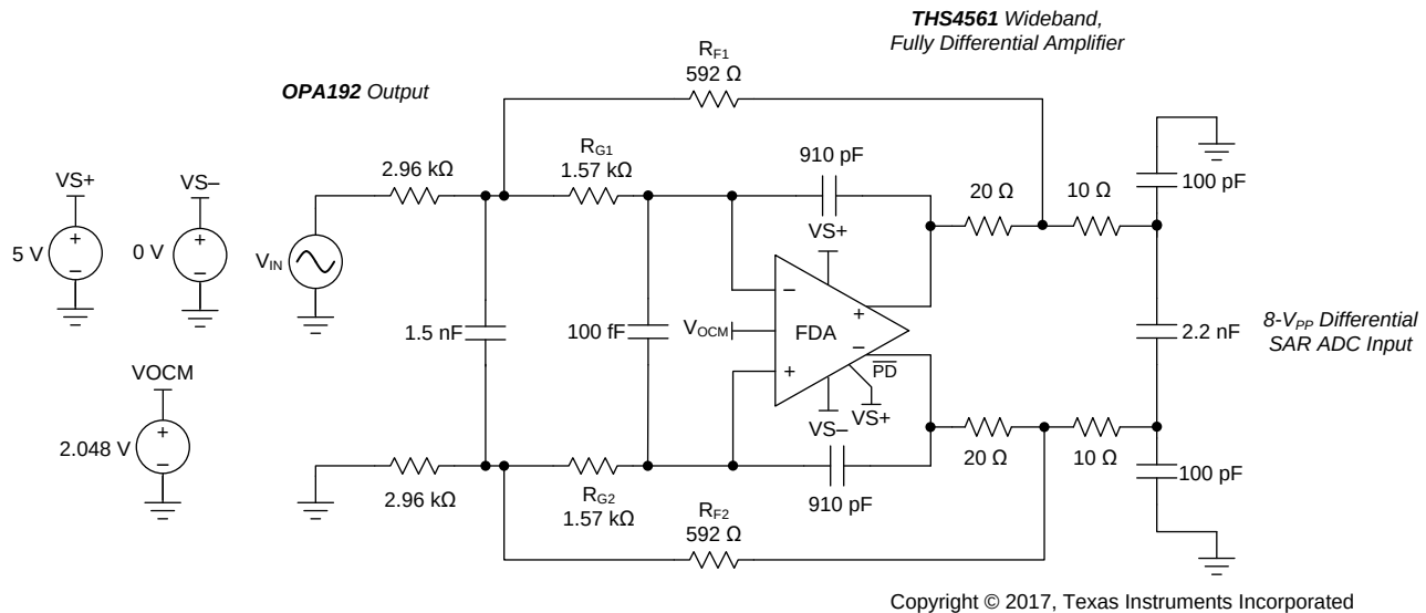
Figure 12. MFB Filter Driving an ADC Application: Example 100-kHz Butterworth Response
