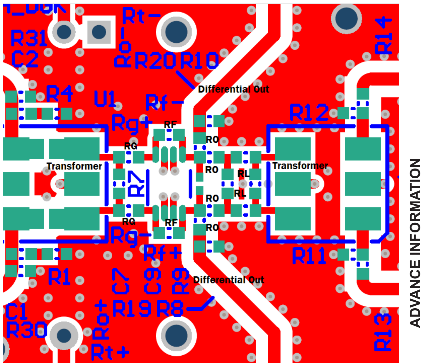
Figure 13. Example Layout
