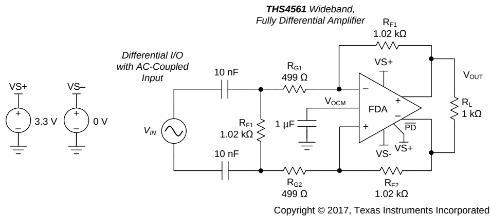
Figure 6. Example AC-Coupled Differential Input Design
