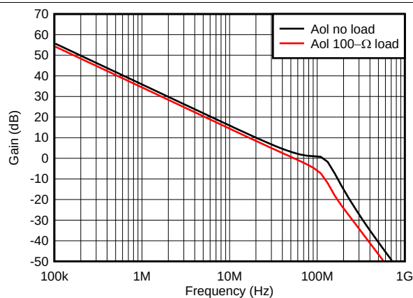
Figure 7. No-Load and 100- \Omega Loaded A_{OL} Gain
