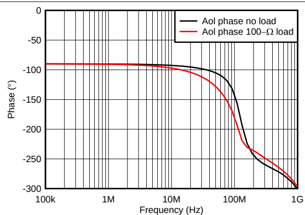
Figure 8. No-Load and 100- \Omega A_{OL} Phase
