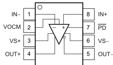
DGK Package 8-Pin VSSOP Top View
