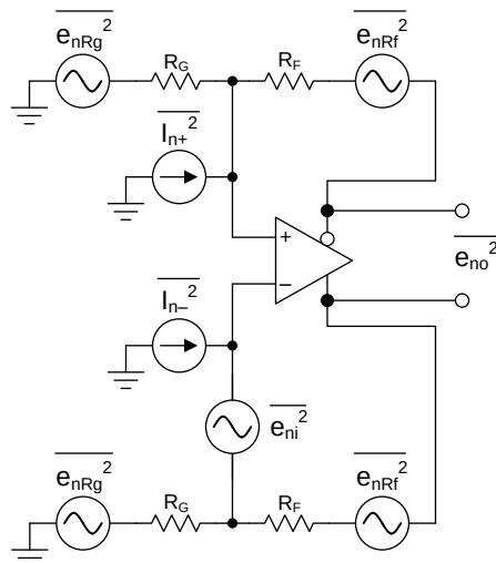
Figure 11. FDA Noise Analysis Circuit
