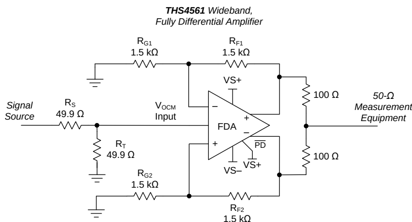
Figure 5. Output Common-Mode Measurements
