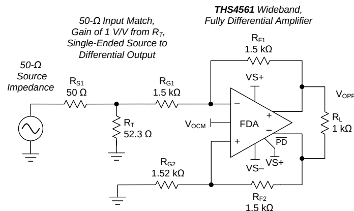
Figure 10. Single-Ended to Differential Gain of 1 V/V with Input Matching Using Standard Resistor Values
