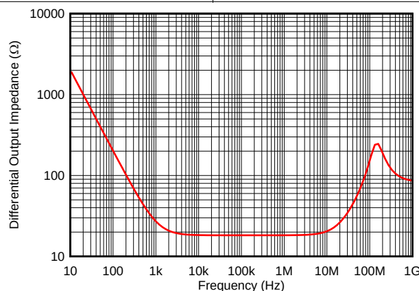
Figure 9. Differential Open-Loop Output Impedance
