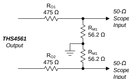
Figure 4. Output Interface for DC-Coupled Differential Outputs
