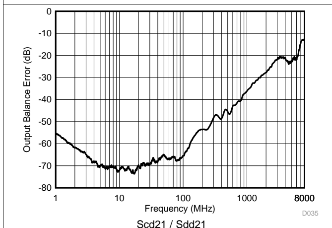
Figure 29. Output Balance Error vs Frequency
