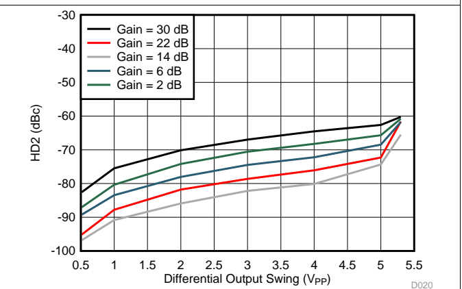
Figure 24. HD2 vs Differential Output Swing (200 MHz)
