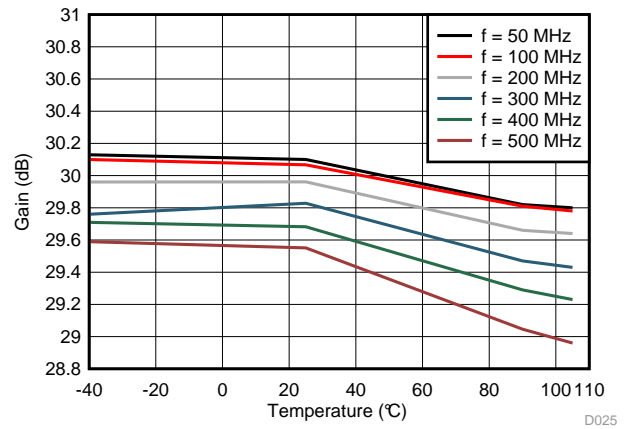
Figure 2. Gain Flatness vs Temperature
