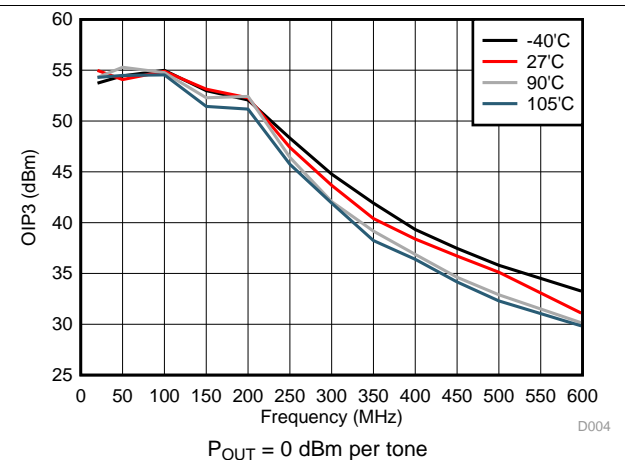
Figure 6. OIP3 vs Frequency and Temperature
