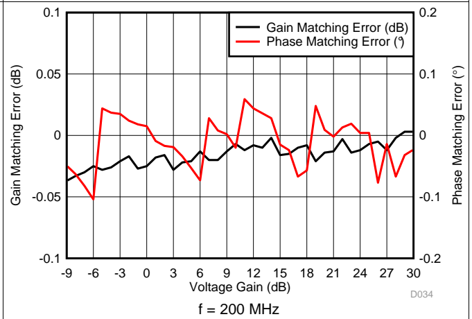
Figure 4. Channel-to-Channel Mismatch Error
