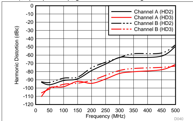
Figure 19. Harmonic Distortion Between Channels
