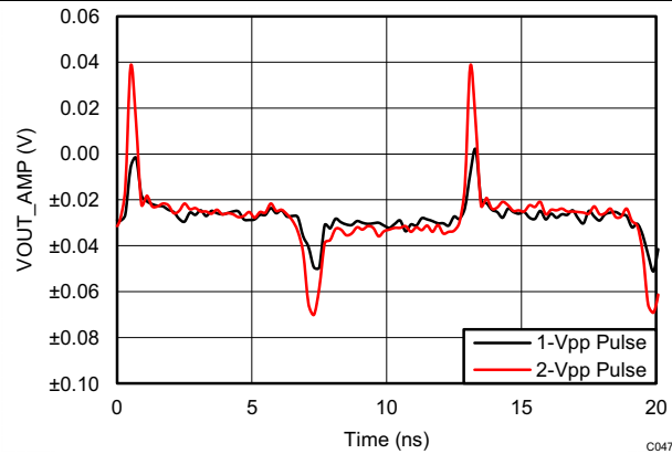
图 52. SE-DE Output Common Mode Pulse Response
