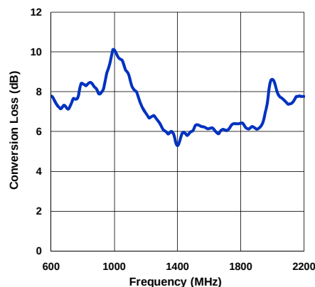
Conversion Loss
